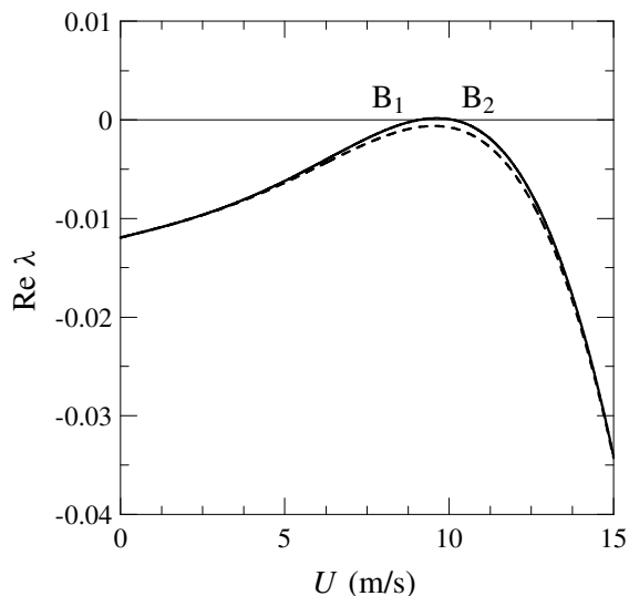
Figure 7. Real part of the critical eigenvalue for CS1 (left) and CS2 (right). Thick lines are used for results obtained with the complete model; dashed lines, for those obtained neglecting the circulatory matrix \mathbf{H} .
