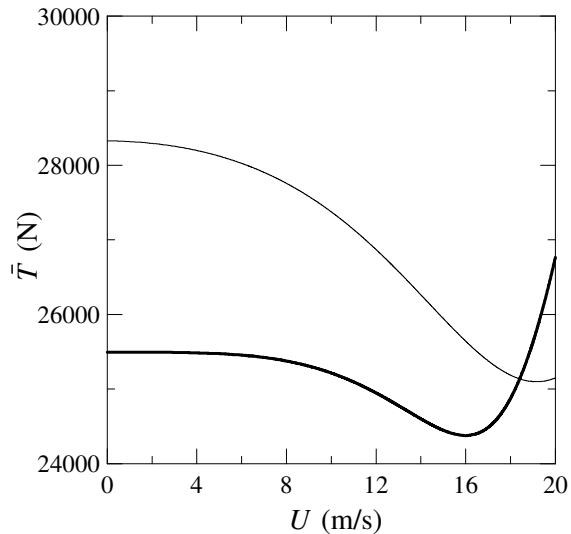
Figure 6. Left: nonlinear equilibrium path \varphi = \varphi(U) for the two different cross-sections in the basic case (thick lines: CS1; thin lines: CS2). Right: changes in the prestress \bar{T} due to the static loads.
