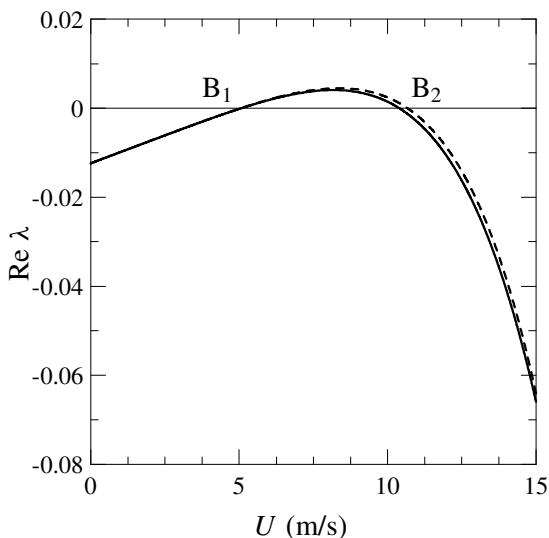
Figure 7. Real part of the critical eigenvalue for CS1 (left) and CS2 (right). Thick lines are used for results obtained with the complete model; dashed lines, for those obtained neglecting the circulatory matrix \mathbf{H} .
