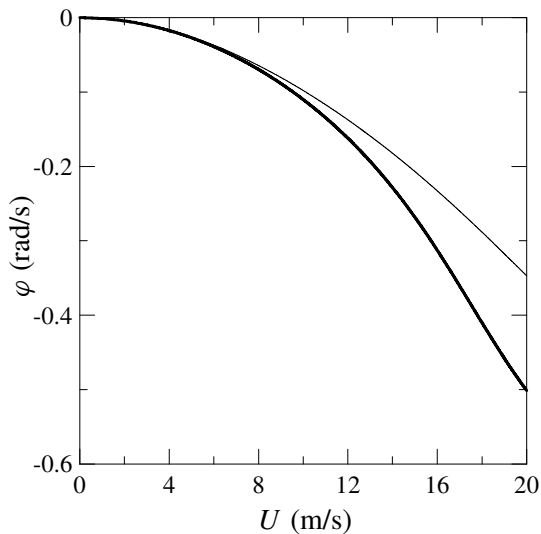
Figure 6. Left: nonlinear equilibrium path \varphi = \varphi(U) for the two different cross-sections in the basic case (thick lines: CS1; thin lines: CS2). Right: changes in the prestress \bar{T} due to the static loads.
