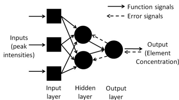
Fig. 1. Schematic of the three-layer artificial neural network used for LIBS analysis with the two basic flows of learning: forward for function signals and backward for errors signals.
