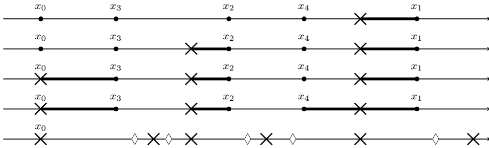
Fig. 3.a - Illustration of the first four steps of Wilson's algorithm in case of killing at x_0 and of (\mathcal{Y}_\infty^{(x_0 \times)}, \mathcal{Z}_\infty^{(x_0 \times)}) : x-dots represent the points of \mathcal{Y}_n^{(x_0 \times)} , diamonds the points of \mathcal{Z}_n^{(x_0 \times)} and thick lines the intervals in \mathcal{J}_n^{(x_0 \times)} .
