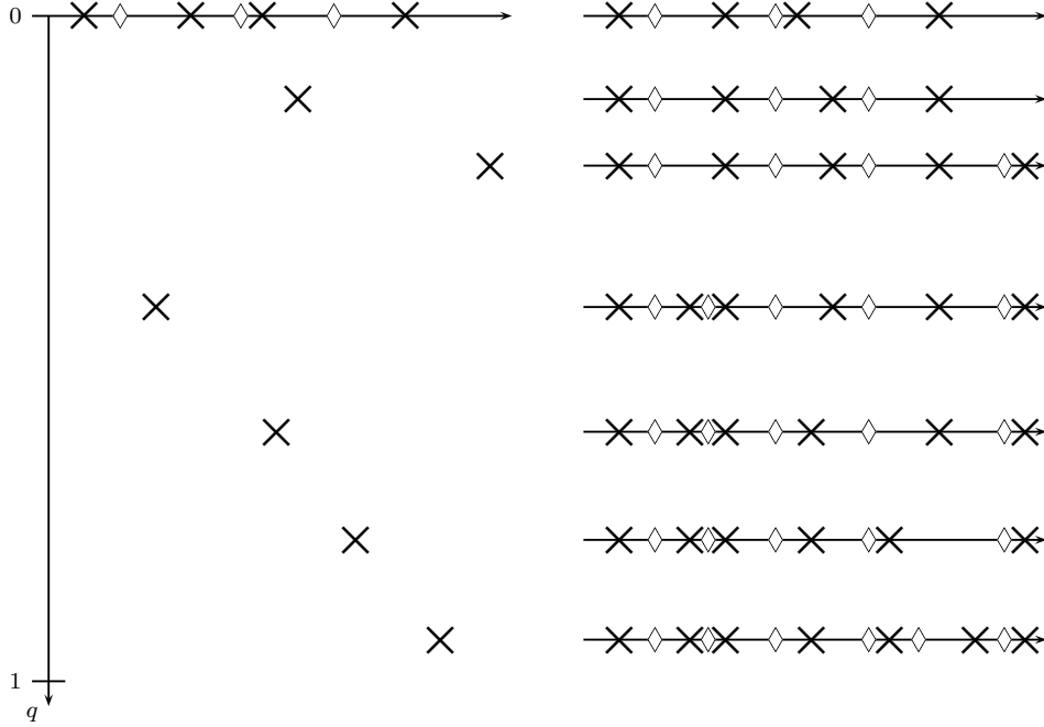
Fig. 4 - Illustration of procedure 7.18: On the left are represented (\mathcal{Y}, \mathcal{Z}) and the Poisson process ((Y_j, q_j))_{1 \leq j \leq N} . On the right are represented the successive ((\mathcal{Y}^{(j)}, \mathcal{Z}^{(j)}))_{0 \leq j \leq N} . x-dots represent the points of \mathcal{Y}^{(j)} and diamonds the points of \mathcal{Z}^{(j)} .
