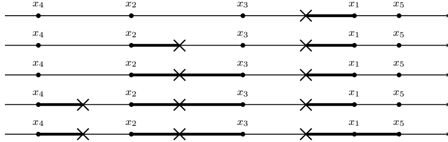
Fig. 2.a - Illustration of ((\mathcal{Y}_n, \mathcal{J}_n))_{1 \leq n \leq 5} : x-dots represent the points of \mathcal{Y}_n and thick lines the intervals in \mathcal{J}_n .
