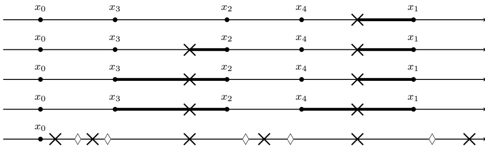
Fig. 3.b - Illustration of the first four steps of Wilson's algorithm in case of reflection at x_0 and of (\mathcal{Y}_\infty^{(x_0 \triangleright)}, \mathcal{Z}_\infty^{(x_0 \triangleright)}) : x-dots represent the points of \mathcal{Y}_n^{(x_0 \triangleright)} , diamonds the points of \mathcal{Z}_n^{(x_0 \triangleright)} and thick lines the intervals in \mathcal{J}_n^{(x_0 \triangleright)} .
