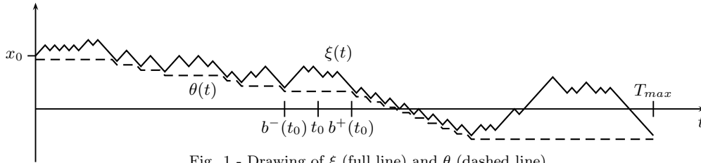
Fig. 1 - Drawing of \xi (full line) and \theta (dashed line).
