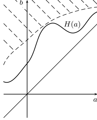
Fig. 2 - The measure on (\min \gamma, \max \gamma) induced by \mu_L^*(d\gamma) is not locally finite in the dashed region.
