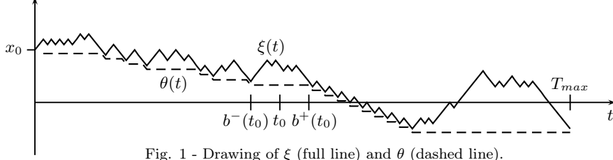
Fig. 1 - Drawing of \xi (full line) and \theta (dashed line).
