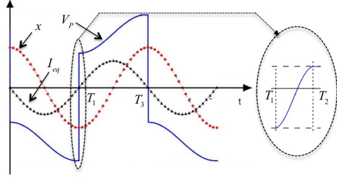
Fig. 8. Waveform of the SSHI piezoelectric energy harvesting device
