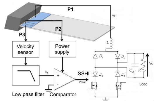
Fig. 11. Experimental setup and circuit diagram of V-SSHI device
