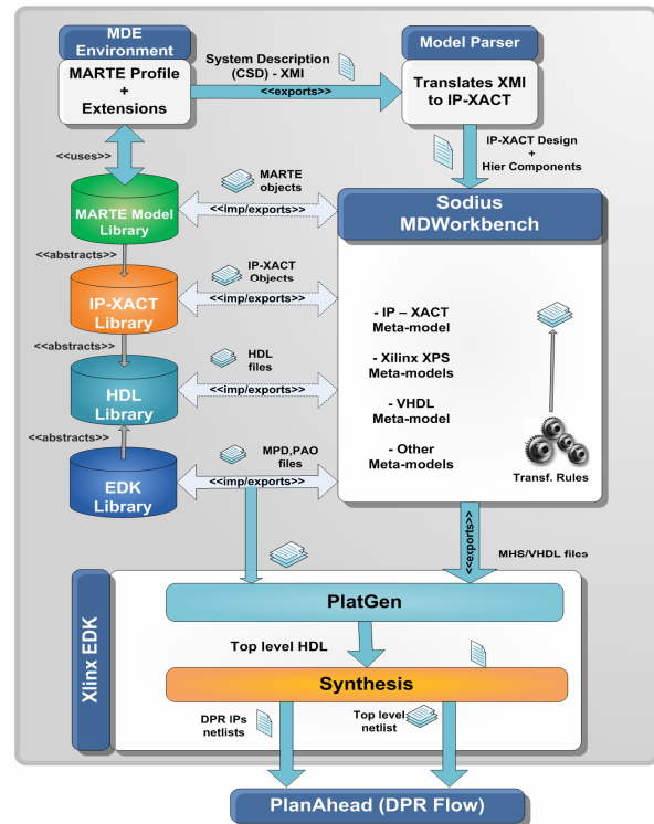
Fig 1. MDE framework for DPR system and IP composition
