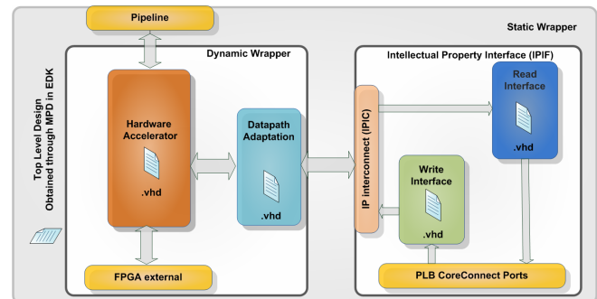
Fig 4. IP-XACT abstract representation for the DPR IP
