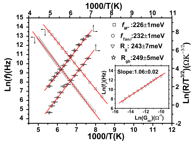
FIG. 4. Arrhenius plots of \tan\delta relaxation frequency, modulus relaxation frequency, grain resistivity, and grain boundary resistivity at DR2 temperature range. The latter two were obtained from the fittings of ECM. The inset is \ln(f_r) vs. \ln(G_{dc}) at low temperature.
