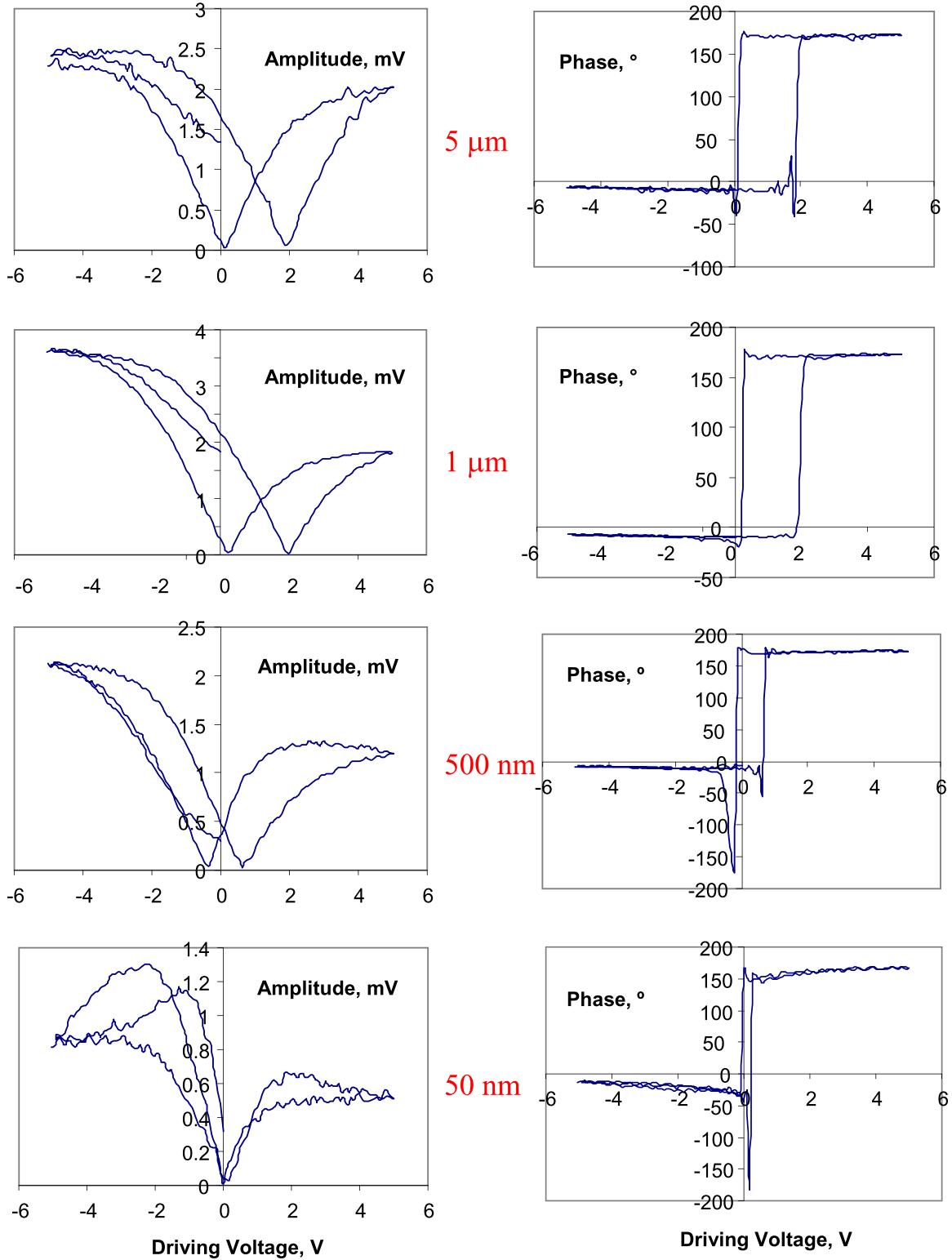
FIG. 3. PFM response amplitude (left) and phase (right) loops of PZT films with micro- and nanometrically sized top electrodes (5 μm, 1 μm, 500 nm, 50 nm from top to bottom).
