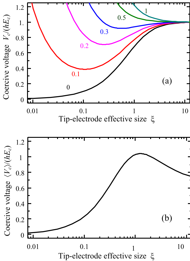
FIG. 4. (a) Local coercive voltages \frac{V_c^{\text{loc}}(0,z)}{E_c h} vs. tip-electrode dimensionless size \xi for different z/h = 0, 0.1, 0.2, 0.3, 0.5, 1 (numbers near the curves). (b) Effective coercive voltage, i.e., V_c^{\text{loc}}(\rho, z) averaged over the PFM response volume \sim (\gamma d)^3 as \langle V_c^{\text{loc}}(\rho, z) \rangle = \frac{1}{\pi^2 \xi^2} \int_0^{\xi} dz \int_0^{\xi} \rho d\rho V_c^{\text{loc}}(\rho, z) \sim \frac{1}{\gamma d} \int_0^{\xi} dz V_c^{\text{loc}}(0, z) .
