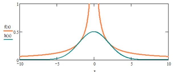
Fig. 7: The same as for the Fig. 6, but \sigma decreased.
