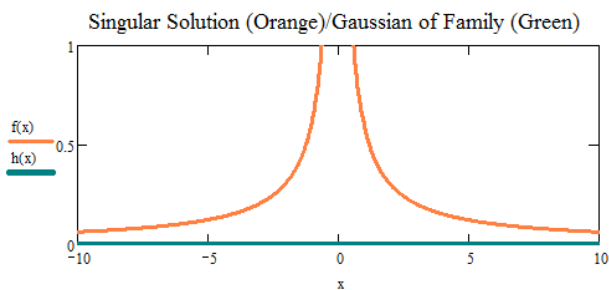
Fig. 1: Eq. (236) [Orange], were we have renamed: \hat{\beta}_k \equiv f , and \xi \equiv x . Eq. (256) [Green], were we have renamed: s \equiv h , and \xi \equiv x . We have taken \tau = 0 . \sigma \rightarrow \infty .
