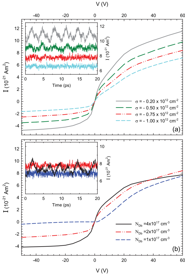
FIG. 2. I - V curves of the GaN SSDs ( L = 1 \mu\text{m} , W = 150 \text{ nm} , W_{\text{V}} = 200 \text{ nm} , W_{\text{H}} = 100 \text{ nm} , and C = 600 \text{ nm} ) when varying: (a) the surface charge density \sigma (for N_{\text{Db}} = 2 \times 10^{17} \text{ cm}^{-3} ) and (b) the background doping N_{\text{Db}} (for \sigma = -0.75 \times 10^{12} \text{ cm}^{-2} ). The plotted value of the current is obtained as the time average for long simulations, including a large enough number of periods when oscillations are present. The insets show current sequences calculated for an applied voltage of 50 V.
