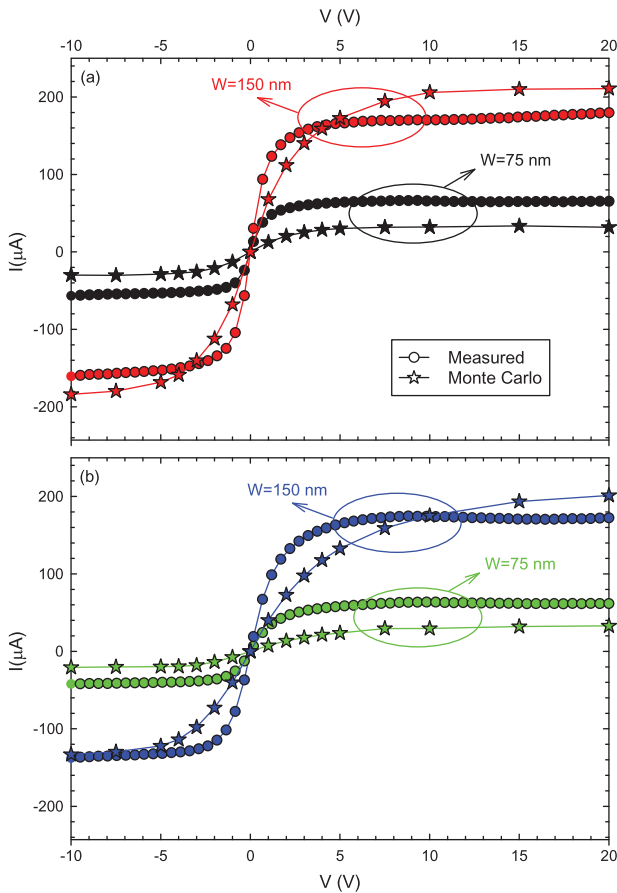
FIG. 10. Comparison between experimental and simulated I - V curves of SSDs with channel length (a) 1 \mu\text{m} and (b) 2 \mu\text{m} ( W_V = 100 \text{ nm} , W_H = 50 \text{ nm} , and C = 400 \text{ nm} ). The self-consistent charge model is used with n_s = 8 \times 10^{12} \text{ cm}^{-2} and N_{\text{Db}} = 1 \times 10^{17} \text{ cm}^{-3} .
