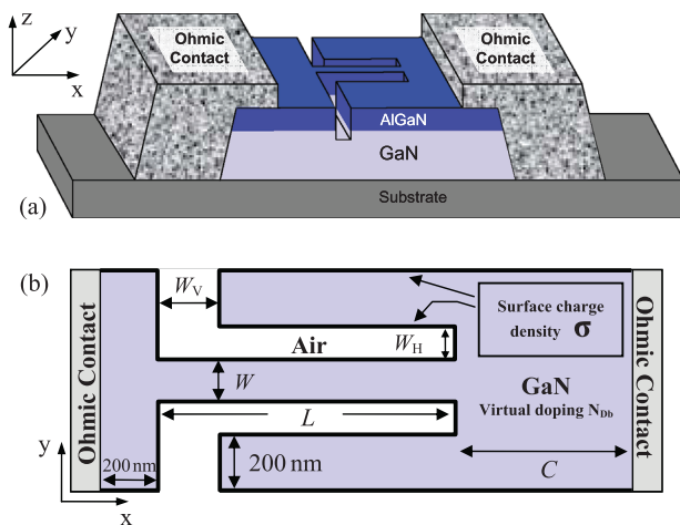
FIG. 1. (a) Typical geometry of SSDs and (b) scheme of the top-view simulations of the GaN channel with the involved parameters (“virtual” doping N_{Db} and negative surface charge density \sigma ). L and W are the length and width of the channel, respectively, W_H the width of the horizontal trenches, W_V the width of the vertical trenches, and C the length of the access region.
