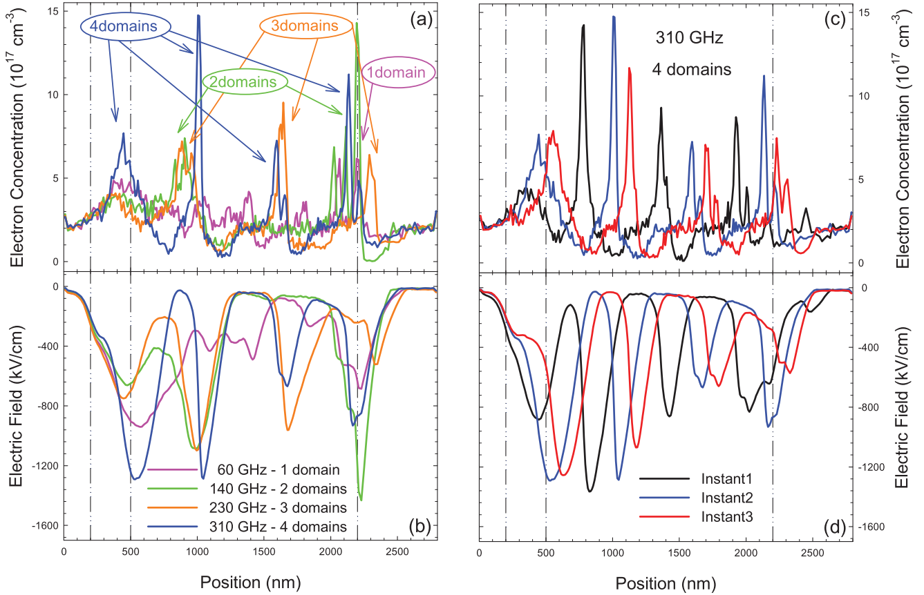
FIG. 6. Profiles of (a) and (c) carrier concentration and (b) and (d) electric field along the centre of the channel of one SSD at room temperature for V_{DC} = 100 V and V_{AC} = 7 V. Curves in (a) and (b) correspond to a given time within one period of the AC signal for frequencies at the center of the emission bands observed in Fig. 5 (60, 140, 230, and 310 GHz). In (c) and (d), they correspond to equidistant time moments during one period of the AC excitation of frequency 310 GHz. The diode has L = 2 \mu\text{m} , W = 150 nm, W_V = 300 nm, W_H = 100 nm, C = 600 nm, \sigma = -0.2 \times 10^{12} \text{cm}^{-2} , and N_{DB} = 2 \times 10^{17} \text{cm}^{-3} . Vertical lines indicate the position of the vertical trenches and the end of the channel.
