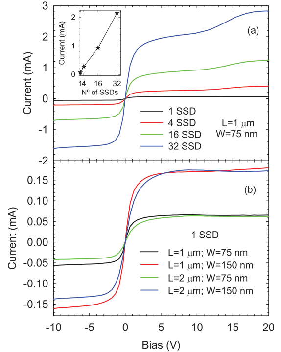
FIG. 8. Experimental I - V characteristics of (a) arrays of SSDs with different number of diodes in parallel with L = 1 \mu\text{m} and W = 75 nm, and (b) of a single SSD with different lengths and widths (all with W_v = 100 nm, W_H = 50 nm, and C = 400 nm). The inset in (a) shows the current for an applied bias of 10 V as a function of the number of SSDs in parallel.
