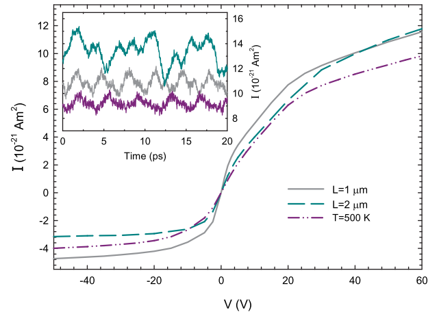
FIG. 3. I-V curves of the GaN simulated SSDs ( \sigma = -0.2 \times 10^{12} \text{ cm}^{-2} , N_{\text{Db}} = 2 \times 10^{17} \text{ cm}^{-3} , W = 150 \text{ nm} , and W_{\text{H}} = 100 \text{ nm} ) when varying the channel length L and the temperature (for L = 1 \mu\text{m} ). The inset show current sequences calculated for an applied voltage of 50 V (100 V for L = 2 \mu\text{m} ).
