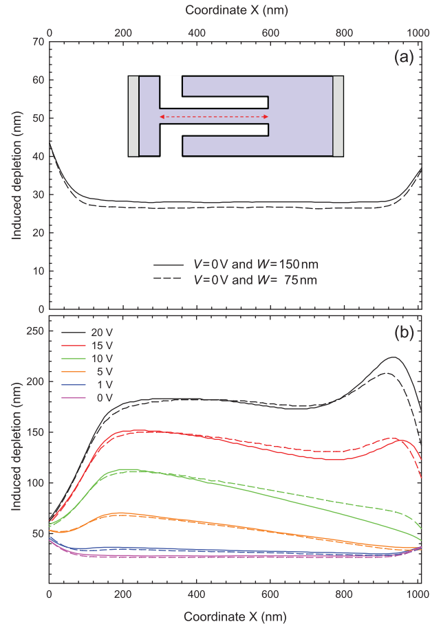
FIG. 11. Profiles of theoretical induced depletion W_d = \sigma/N_{\text{Db}} originated by the surface charge in the diodes of 1 \mu\text{m} length and two different widths ( W = 75 and 150 \text{ nm} ). (a) Equilibrium conditions. (b) Positive applied voltages. Solid lines correspond to W = 150 \text{ nm} and dashed lines to W = 75 \text{ nm} .
