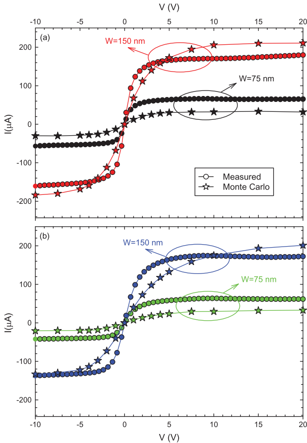
FIG. 10. Comparison between experimental and simulated I - V curves of SSDs with channel length (a) 1 \mu\text{m} and (b) 2 \mu\text{m} ( V_{\text{H}} = 100 \text{ nm} , W_{\text{H}} = 50 \text{ nm} , and C = 400 \text{ nm} ). The self-consistent charge model is used with n_s = 8 \times 10^{12} \text{ cm}^{-2} and N_{\text{Db}} = 1 \times 10^{17} \text{ cm}^{-3} .
