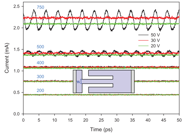
FIG. 12. Current sequences for diodes with different widths and applied voltages of 20, 30, and 50 V. The channel length is 1 \mu\text{m} and the temperature of operation is 300 K. The numbers in the graph correspond to W in nm. The chosen value for n_s is 8 \times 10^{12} \text{ cm}^{-2} .
