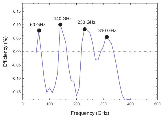
FIG. 5. DC to AC conversion efficiency \eta as a function of the frequency of the AC excitation for a diode with L = 2 \mu\text{m} , W = 150 \text{ nm} , W_V = 300 \text{ nm} , W_H = 100 \text{ nm} , C = 600 \text{ nm} , \sigma = -0.2 \times 10^{12} \text{ cm}^{-2} , N_{Db} = 2 \times 10^{17} \text{ cm}^{-3} , and T = 300 \text{ K} . V_{DC} = 100 V, and V_{AC} = 7 V.
