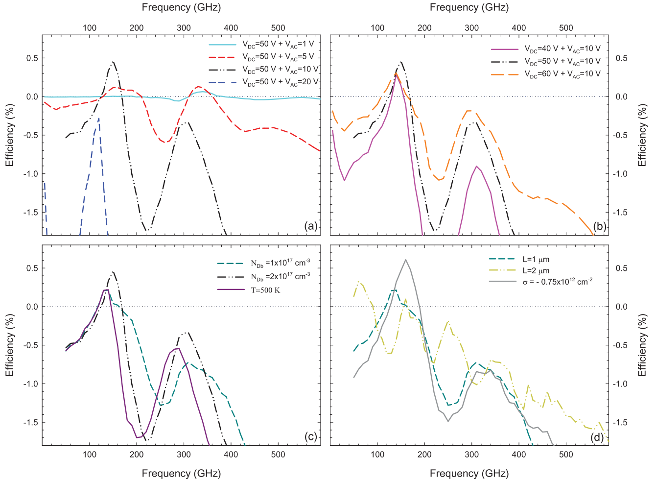
FIG. 4. DC to AC conversion efficiency \eta as a function of the frequency of the AC excitation when varying: (a) the AC bias conditions ( V_{DC} = 50 V), (b) the DC bias conditions ( V_{AC} = 10 V), (c) background doping N_{Db} and temperature T , and (d) channel length L and surface charge \sigma ( N_{Db} = 1 \times 10^{17} \text{ cm}^{-3} ). Unless otherwise indicated, L = 1 \mu\text{m} , W = 150 \text{ nm} , W_V = 200 \text{ nm} , W_H = 100 \text{ nm} , C = 600 \text{ nm} , \sigma = -0.2 \times 10^{12} \text{ cm}^{-2} , N_{Db} = 2 \times 10^{17} \text{ cm}^{-3} , and T = 300 \text{ K} . In (c) and (d), V_{DC} = 50 V and V_{AC} = 10 V (except for the case L = 2 \mu\text{m} , for which V_{DC} = 100 V and V_{AC} = 20 V).
