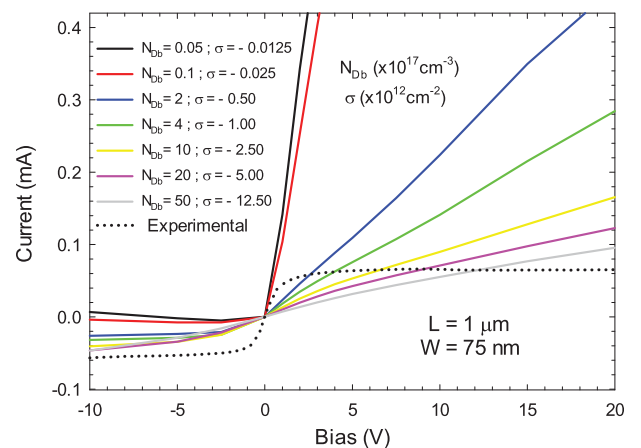
FIG. 9. Comparison between measured and simulated I - V curves for a diode with L = 1 \mu\text{m} and W = 75 nm with different sets of values of N_{\text{Db}} and \sigma providing the same W_d = \sigma/N_{\text{Db}} = 25 nm.
