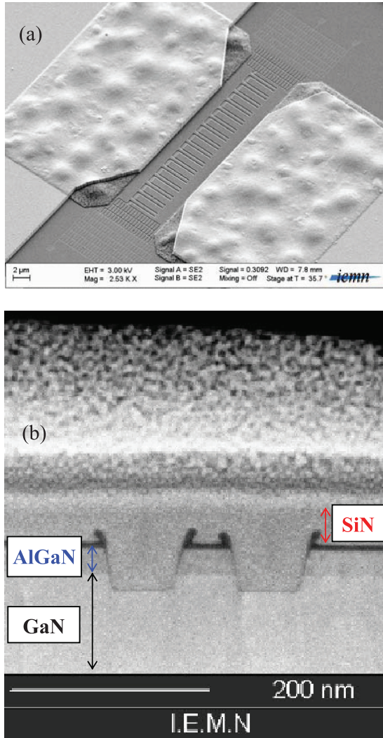
FIG. 7. (a) SEM image of an array of 16 SSDs in parallel and (b) FIB cut view showing the shape of the recess.
