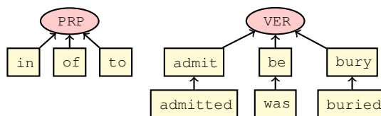
Figure 5: Items Hierarchy
