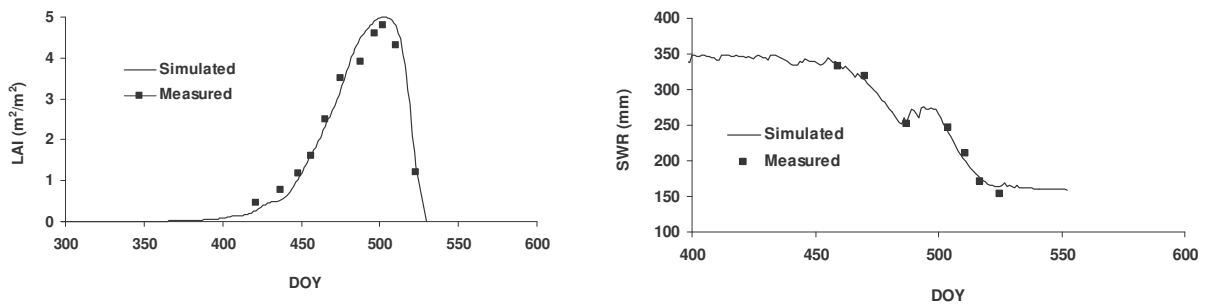
Fig. 3: Simulations of LAI and SWR in the rainfed treatment in 2010 with the Ce and RMSE criteria (LAI: Ce=0.962 and RMSE=0.31 m 2 /m 2 ; SWR: Ce=0.988 and RMSE=6.7 mm).
