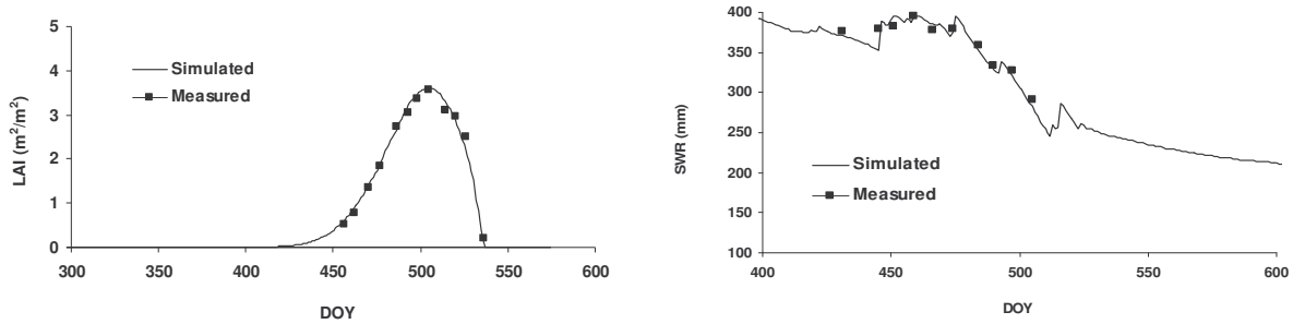
Fig. 2: Simulation of LAI and SWR in 2008-2009 with the Ce and RMSE criteria (LAI: Ce=0.986 and RMSE=0.13 m 2 /m 2 ; SWR: Ce=0.875 and RMSE=11.47 mm).
