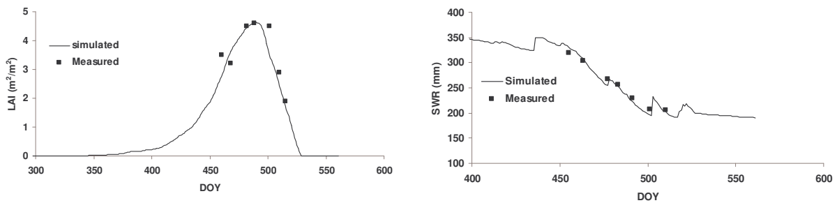
Fig. 4: Simulations of LAI and SWR in an agricultural field (WAD = 43 mm on 05/18) in 2010-2011 crop season (LAI: Ce=0.676 and RMSE=0.53 m 2 /m 2 ; SWR: Ce=0.962 and RMSE=8 mm).
