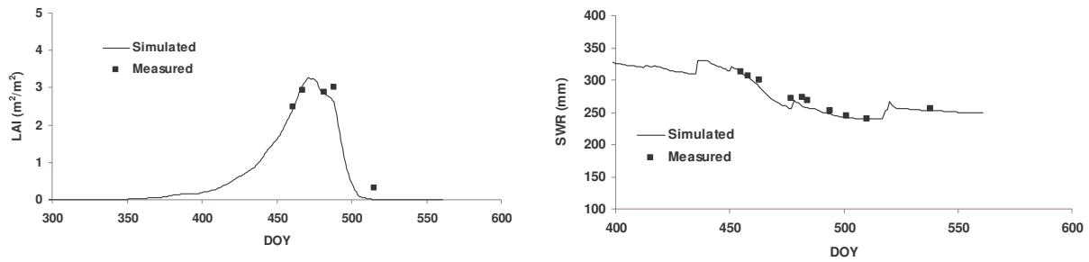
Fig. 5: Simulations of LAI and SWR in a rainfed agricultural field in 2010-2011 crop season (LAI: C_e=0.952 and RMSE=0.21 \text{ m}^2/\text{m}^2 ; SWR: C_e=0.870 and RMSE=9 \text{ mm} ).
