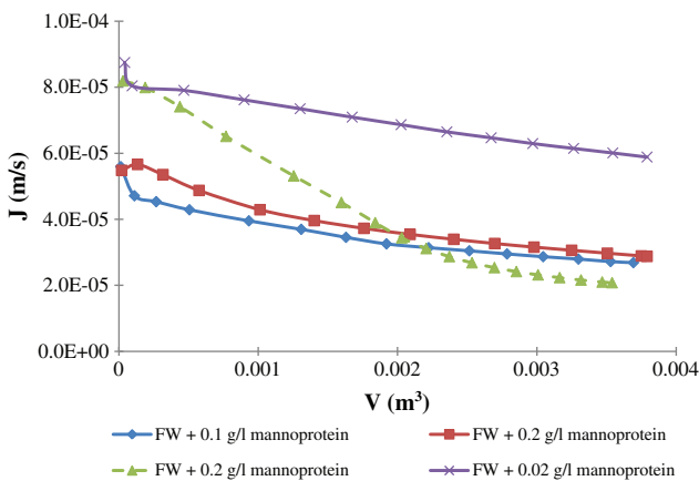
Fig. 10. Permeate fluxes versus permeate volume during wine filtration added with mannoproteins (—: 0.5 \times 10^5 Pa; ---: 1 \times 10^5 Pa).
