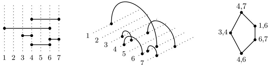
FIGURE 2. The heap m = x_{46}x_{67}x_{34}x_{16}x_{47} as a pile of segments and the Hasse diagram of the associated poset.
