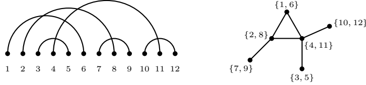
FIGURE 1. A matching \sigma and its crossing graph G(\sigma) .
