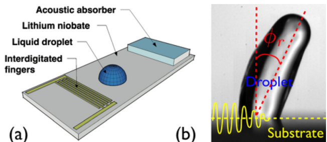
FIG. 1. (a) Sketch of the experimental setup. (b) Drop undergoing large deformation along the acoustic wave refraction angle \phi_r .
