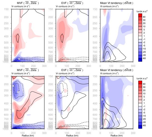
FIG. 6. Vertical cross sections of the mean (MVF) and eddy (EVF) vorticity flux terms in the tangential wind budget equation, as well as the tangential wind tendency (right panel), after 29h- (top) and 36h- (bottom) integration. Shading contours are indicated in the legendbar. The contours superimposed are mean radial velocity (MVF and EVF panels) and tangential wind (right plot).
