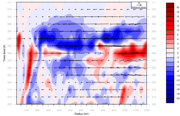
FIG. 5. Radius-theta cross section of EP flux vectors and their divergence (shaded) after 38h-integration. The divergence contour interval is 10^4 \text{ Pa m}^2 \text{ K}^{-1} \text{ s}^{-2} ; horizontal and vertical arrow scales are 1.3 \times 10^8 \text{ Pa m}^3 \text{ K}^{-1} \text{ s}^{-2} and 9.3 \times 10^2 \text{ Pa m}^2 \text{ s}^{-2} (reference indicated in legend).
