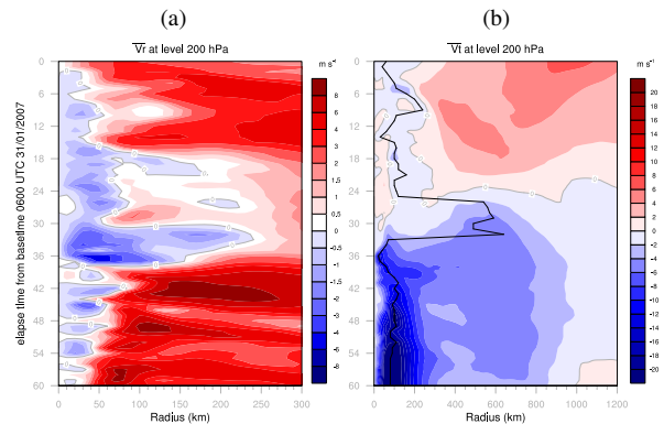
FIG. 3. Radius-time series of the 200 hPa azimuthally averaged (a) radial and (b) tangential velocity during the Aladin forecast of DORA. Radii go out to 300 km in (a) and 1200 km in (b). The black line in (b) indicates the radius where the cyclonic tangential wind are maximum.
