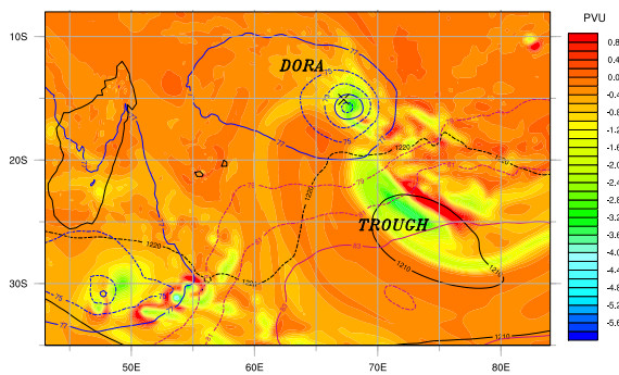
FIG. 2. Ertel potential vorticity on the 330 K isentropic surface (shading, in \text{PVU} \equiv 10^{-6} \text{ m}^2 \text{ K s}^{-1} \text{ kg}^{-1} ) for TC Dora at 0600 UTC 1 February 2007 in the ECMWF operational analysis at 0.25^\circ -resolution. Contours are geopotential height at levels 925 hPa (blue and purple lines, mgp) and 200 hPa (black lines, mgp). The cross indicates Dora’s best track center.
