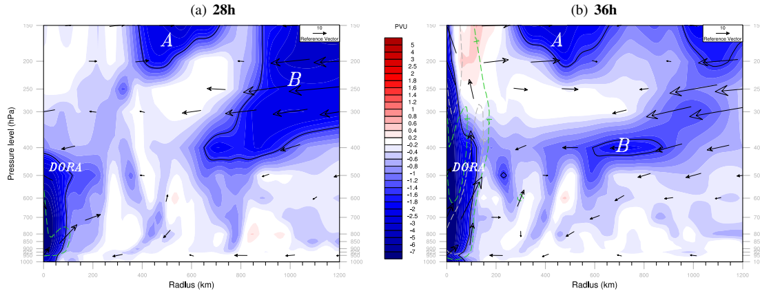
FIG. 4. Vertical cross sections of the PV (shaded, with the -1.5 PVU contour blackened) from the TC center to the south-southeast after (a) 28h- and (b) 36h-integration. Arrows show radial and vertical ( -10 \cdot \omega ) velocity above 5 \text{ m s}^{-1} (reference arrow indicated in legend). Dashed green (gray) contours indicate the regions where \omega is less than -1 . ( -2 ) \text{Pa s}^{-1} .
