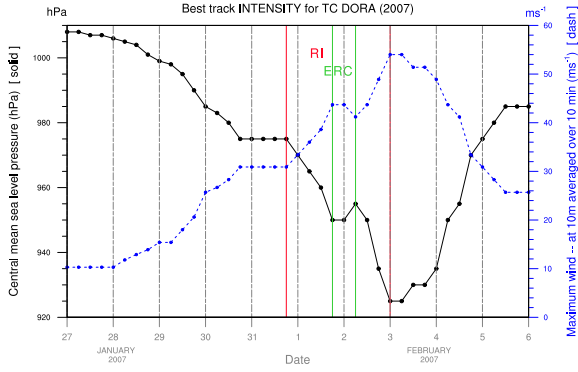
FIG. 1. Best track data for Dora (27 Jan-06 Feb 2007): central pressure (solid black line, left axis, hPa) and maximum wind speed (dashed blue line, right axis, \text{m s}^{-1} ).
