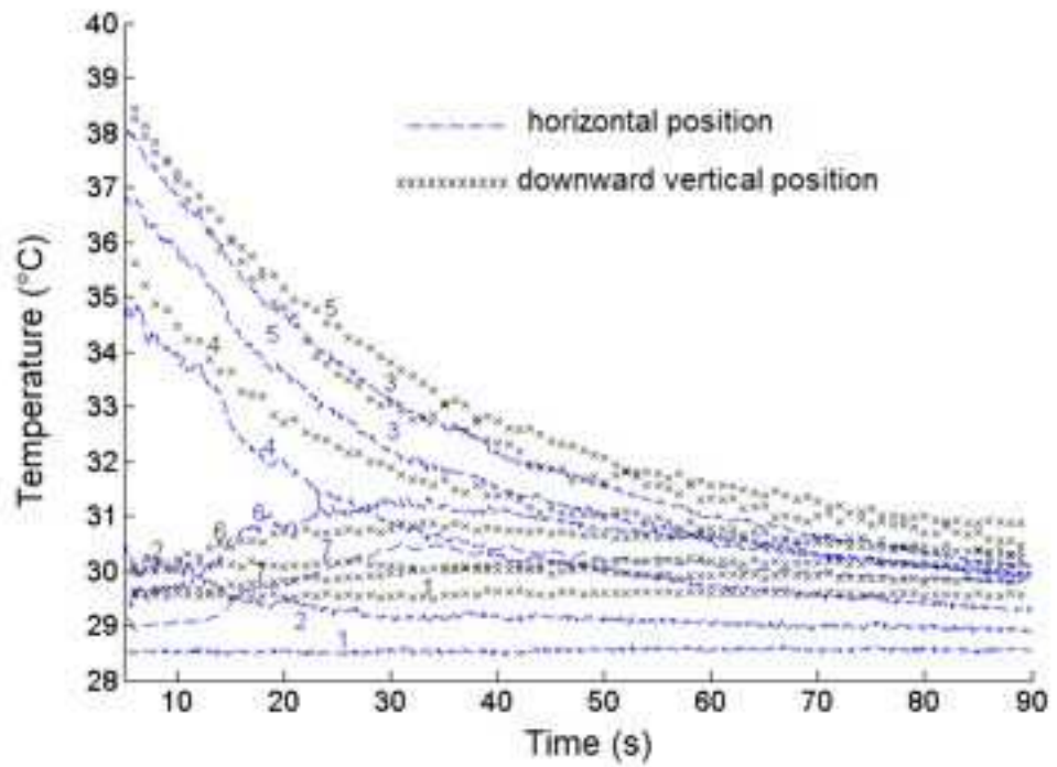
Figure 12: Comparison of experimental results between horizontal and downward vertical positions: female subject - cooled bar (top) and heated bar (bottom)
