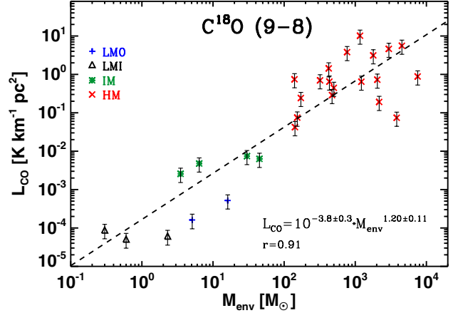
Fig. 7. \text{C}^{18}\text{O } J = 9-8 line luminosity for low-mass Class 0 (LM0; blue pluses), low-mass Class I (LMI; black triangles), intermediate-mass (IM; green asterisks) and high-mass (HM; red crosses) YSOs versus their envelope masses, M_{\text{env}} . The dash black line represents the linear function that fits the logarithm of the plotted quantities.
