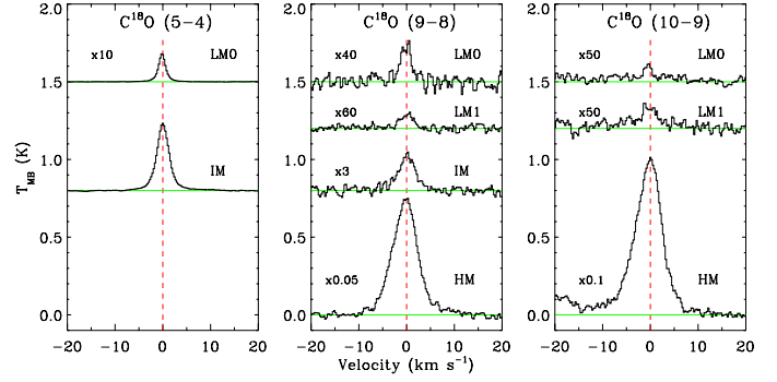
Fig. 11. Same as Fig. 10 but for the \text{C}^{18}\text{O} spectra from the observed transitions: J=5-4 (left), J=9-8 (centre) and J=10-9 (right). More details about these transitions are in Appendix A.
