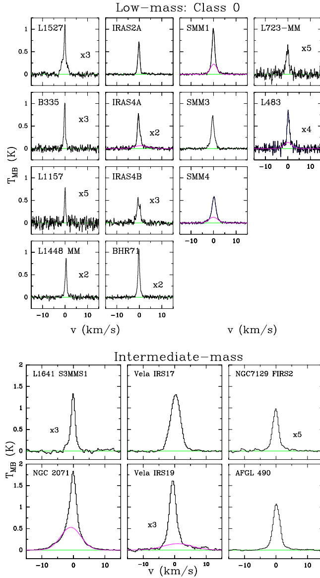
Fig. A.3. Same as Fig. A.1 but for the C^{18}O J = 5-4 spectra of the low-mass (Class 0) and intermediate-mass protostars. For the low-mass sample the HRS spectra are presented, while the WBS data is used for the intermediate-mass objects.
