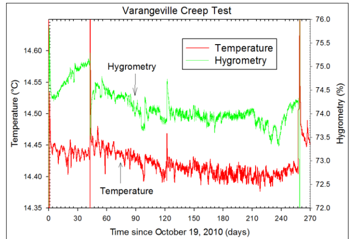
Figure 6. Temperature and hygrometry of the gallery air from day 1 to day 260.
