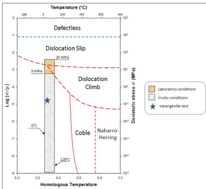
Figure 1. Mechanism map (after Munson & Dawson 1984).
