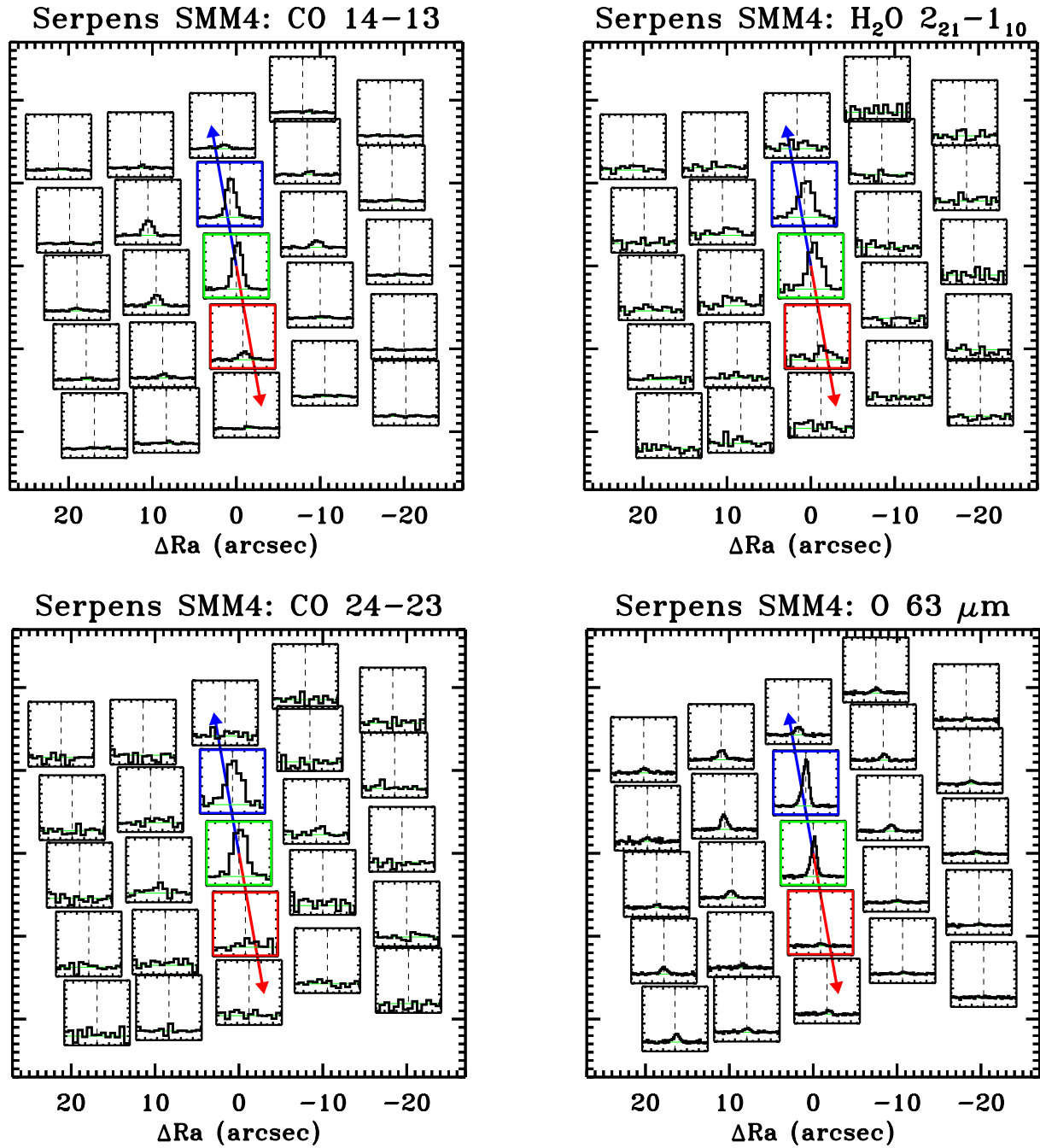
Fig. J.8. Ser SMM4 maps in the [O I] ^3P_1-^3P_2 line at 63.2 \mu\text{m} , the H 2 O 2 21 -1 10 at 108.1 \mu\text{m} , the CO 14-13 at 186.0 \mu\text{m} , and the CO 24-23 at 108.7 \mu\text{m} .
