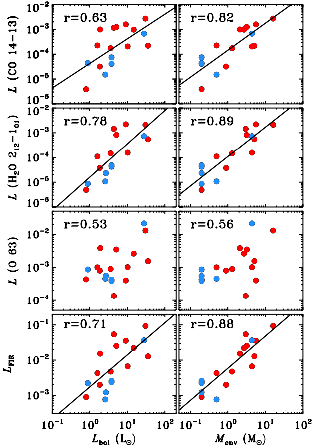
Fig. 10. Correlations of full array line emission with bolometric luminosity (left column) and envelope mass (right column) from top to bottom: CO 14–13, H 2 O 2 12 –1 01 , [O I] at 63.2 \mu m line luminosities, and total far-IR gas cooling L_{\text{FIR}} .
