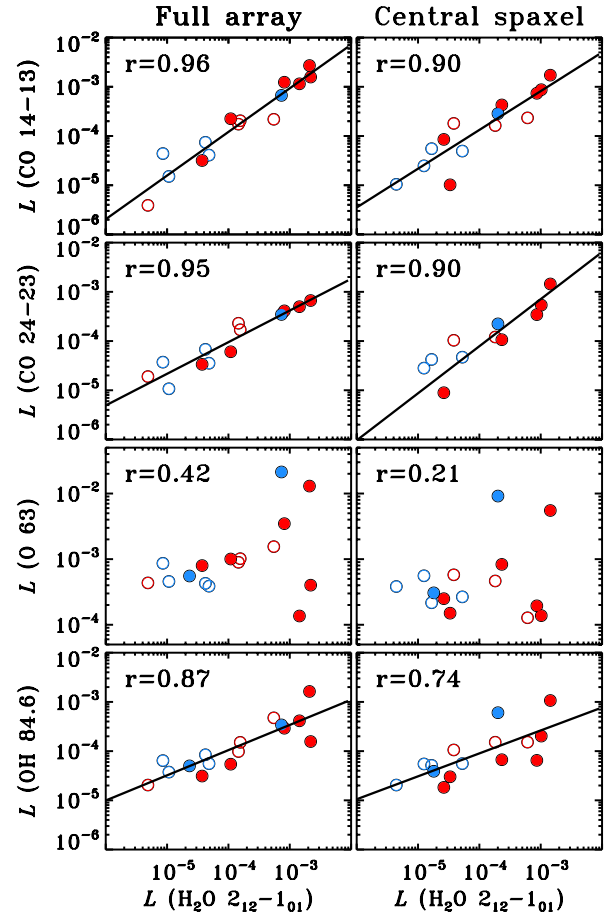
Fig. 9. Luminosity correlations between the \text{H}_2\text{O} 2_{12}\text{--}1_{01} line at 179.527\ \mu\text{m} and (from top to bottom) CO 14–13, CO 24–23, [OI] at 63.18\ \mu\text{m} , and OH at 84.6\ \mu\text{m} , for 16 out of 18 objects (all luminosities in units of L_\odot ). Full array and central spaxel luminosities are shown in the left and right columns, respectively. Red circles correspond to Class 0 sources and blue circles to Class I sources. Empty symbols show the compact sources, whereas filled symbols denote the extended sources. The Pearson coefficient of the correlation ( r ) is shown.
