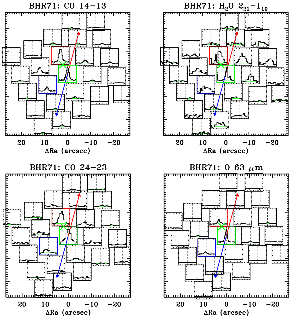
Fig. J.4. BHR71 maps in the [O I] ^3P_1-^3P_2 line at 63.2 \mu\text{m} , the H 2 O 2 21 -1 10 at 108.1 \mu\text{m} , the CO 14-13 at 186.0 \mu\text{m} , and the CO 24-23 at 108.7 \mu\text{m} .
