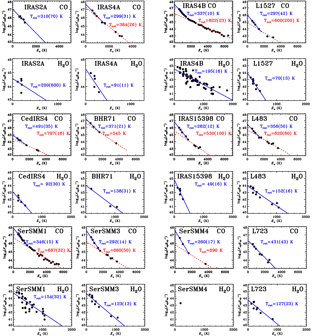
Fig. F.1. Rotational diagrams of CO and H 2 O for Class 0 sources. Blue and red lines show linear fits to warm and hot components, respectively. The corresponding rotational temperatures are written in the same colors. Errors associated with the fit are shown in the brackets. Warm component only is seen towards L723 in our diagram.
