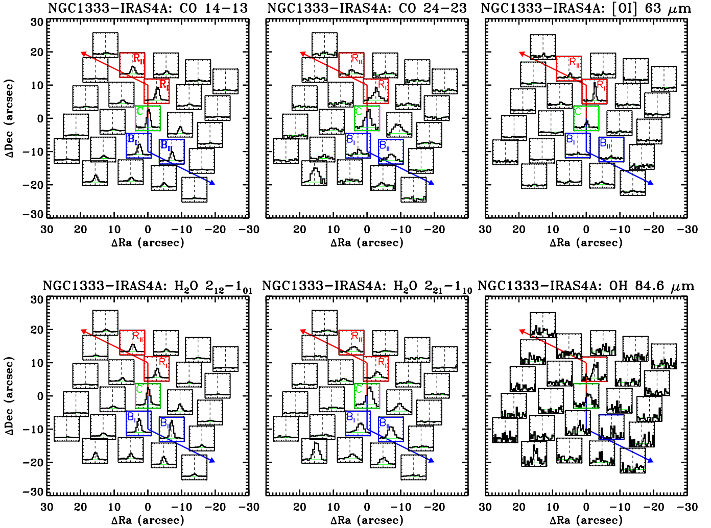
Fig. 3. PACS spectral maps of the Class 0 source NGC 1333-IRAS4A in the CO 14–13, CO 24–23, [OI] 63.2 \mu\text{m} , \text{H}_2\text{O} 2_{12}-1_{01} , \text{H}_2\text{O} 2_{21}-1_{10} and OH 84.6 \mu\text{m} lines. The center of each spaxel box corresponds to its position on the sky with respect to the pointed source coordinates from van Dishoeck et al. (2011); shown boxes are smaller than the actual spaxel sizes. Wavelengths in microns are translated to the velocity scale on the X-axis using laboratory wavelengths of the species and cover the range from -550 to 550 \text{ km s}^{-1} , except for the OH 84.6 \mu\text{m} lines where -400 to 400 \text{ km s}^{-1} is shown. The Y-axis shows fluxes normalized to the brightest spaxel on the map separately for each species in a range -0.2 to 1.2 . Outflow directions are drawn in blue and red lines based on CO 6–5 APEX CHAMP + sub-mm maps (Yıldız et al. 2012, and in prep.) that traces the warm entrained gas ( T \sim 100 \text{ K} ). Two red outflow ( R_1 , R_{II} ), on-source (C) and blue outflow ( B_1 , B_{II} ) spaxels are marked with letters. IRAS4A spectra at those positions in different species are shown in Appendix D. The contribution from NGC 1333-IRAS4B, located at (22.5'', -22.8'') with respect to IRAS4A, is seen in the S-E part of the map.
