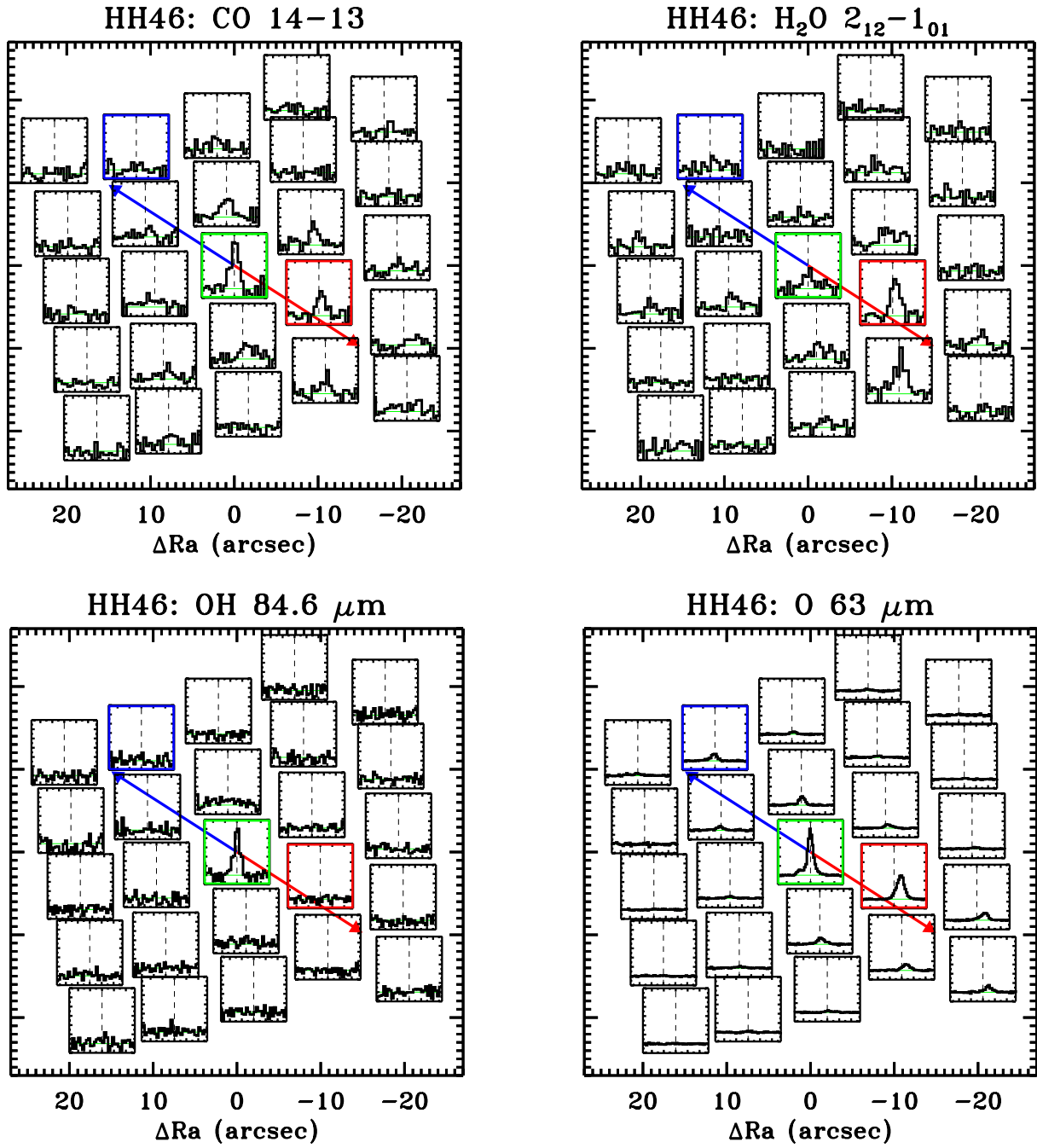
Fig. J.15. HH46 maps in the [O I] ^3\text{P}_1-^3\text{P}_2 line at 63.2 \mu\text{m} , the H 2 O 2 12 -1 01 line at 179.5 \mu\text{m} , the CO 14-13 at 186.0 \mu\text{m} and the OH ^2\Pi_{3/2} J = 7/2-5/2 line at 84.6 \mu\text{m} .
