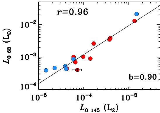
Fig. 11. Full array correlation between the [O I] line luminosities at 145 and 63 \mu m for 16 out of 18 objects (the [O I] 145 line is not detected in NGC 1333-IRAS2A and 4B). Class 0 sources are shown in red and Class I sources in blue. A typical error is shown on the NGC 1333-IRAS4A observation.
