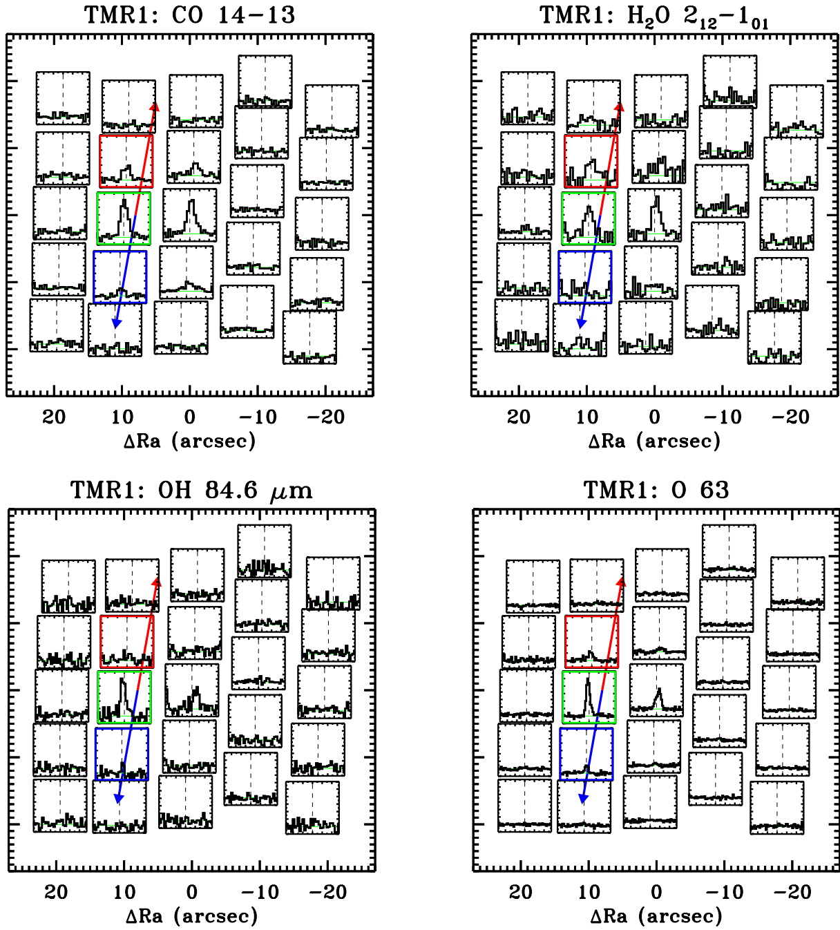
Fig. J.12. TMR1 maps in the [O I] ^3P_1-^3P_2 line at 63.2 \mu\text{m} , the H 2 O 2 12 -1 01 line at 179.5 \mu\text{m} , the CO 14-13 at 186.0 \mu\text{m} and the OH ^2\Pi_{3/2} J = 7/2-5/2 line at 84.6 \mu\text{m} .
