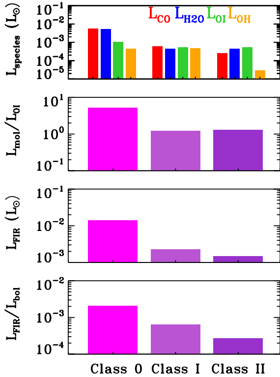
Fig. 15. Panel 1: median cooling in CO, H 2 O, OH, and [O I] lines for Class 0, I, and II objects are shown from left to right for each class in red, blue, orange and green colors, respectively. (Class II data from Podio et al. 2012.). Panel 2: evolution of the ratio of molecular and atomic cooling. Panel 3: evolution of the median total far-IR gas cooling. Panel 4: evolution of the median total far-IR gas cooling over bolometric luminosity.
