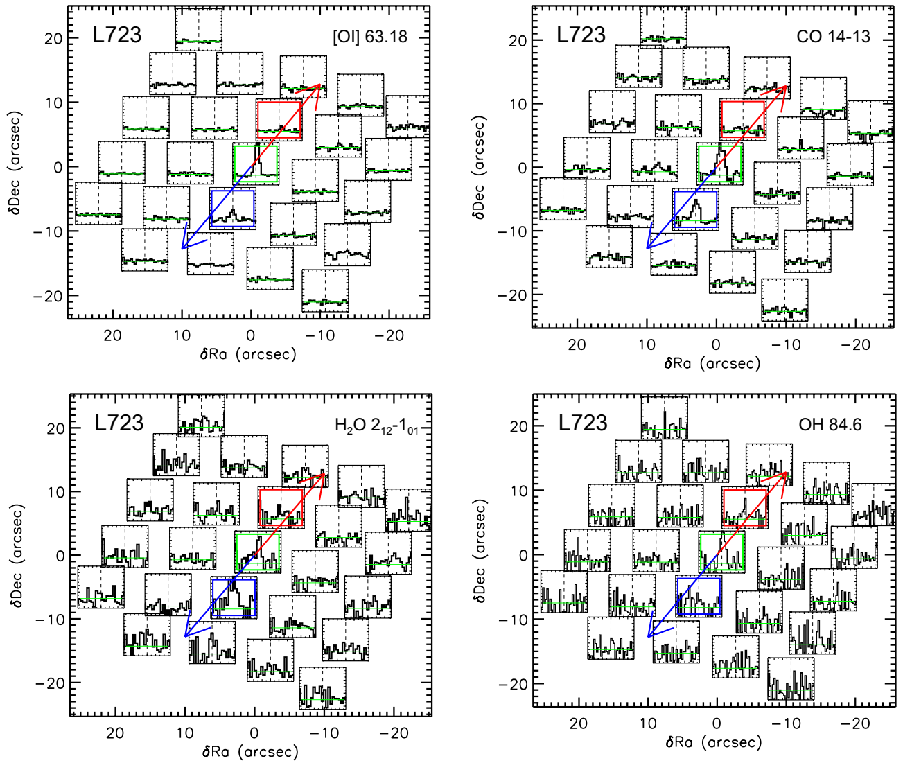
Fig. J.10. L723 maps in the [OI] ^3P_1 - ^3P_2 line at 63.2 \mu\text{m} , the H 2 O 2 12 -1 01 line at 179.5 \mu\text{m} , the CO 14-13 at 186.0 \mu\text{m} , and the OH ^2\Pi_{3/2} J = 7/2 - 5/2 line at 84.6 \mu\text{m} .
