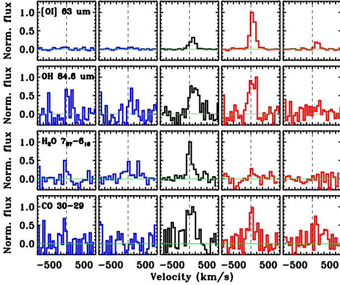
Fig. D.3. NGC 1333-IRAS4A spectra in the [O I] 63.2 \mu\text{m} line, the OH 84.6 \mu\text{m} line, the H 2 O 7 07 –6 16 line, and the CO 30–29 line. Two blue outflow, on-source and two red outflow positions are shown, corresponding to the colored spaxels in Fig. 3.
