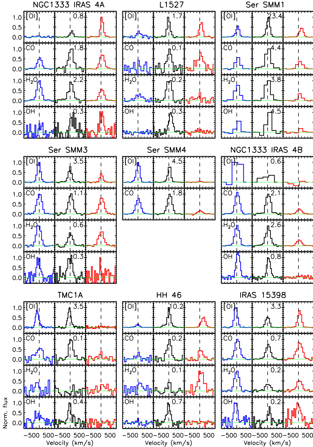
Fig. D.1. Spectra of the [O I] 63.2 \mu\text{m} , CO 14–13 186.0 \mu\text{m} , H 2 O 2 12 –1 01 179.5 \mu\text{m} , and OH 84.6 \mu\text{m} lines in the selected blue outflow, on-source and red outflow positions (marked with blue, green and red frames around the spaxels e.g. in Fig. 3) for the extended sources (see Sect. 3.2). The figure shows relative emission at different positions for each species separately. Measured line fluxes at central spaxel position in units of 10^{-20} \text{ W cm}^{-2} are written next to the corresponding spectra.
