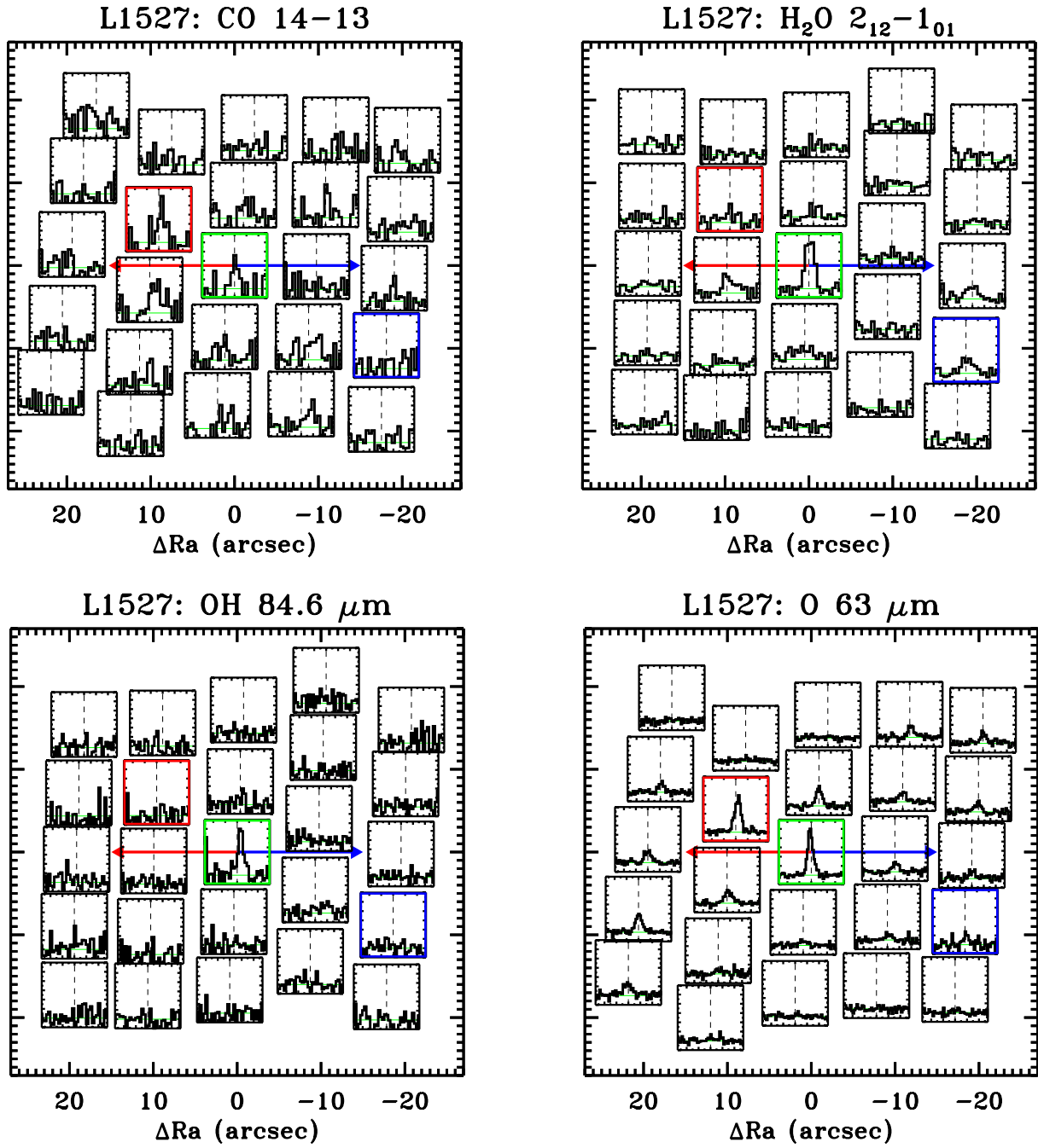
Fig. J.2. L1527 maps in the [O I] ^3P_1 - ^3P_2 line at 63.2 \mu\text{m} , the H 2 O 2 12 -1 01 line at 179.5 \mu\text{m} , the CO 14-13 at 186.0 \mu\text{m} , and the OH ^2\Pi_{3/2} J = 7/2 - 5/2 line at 84.6 \mu\text{m} .
