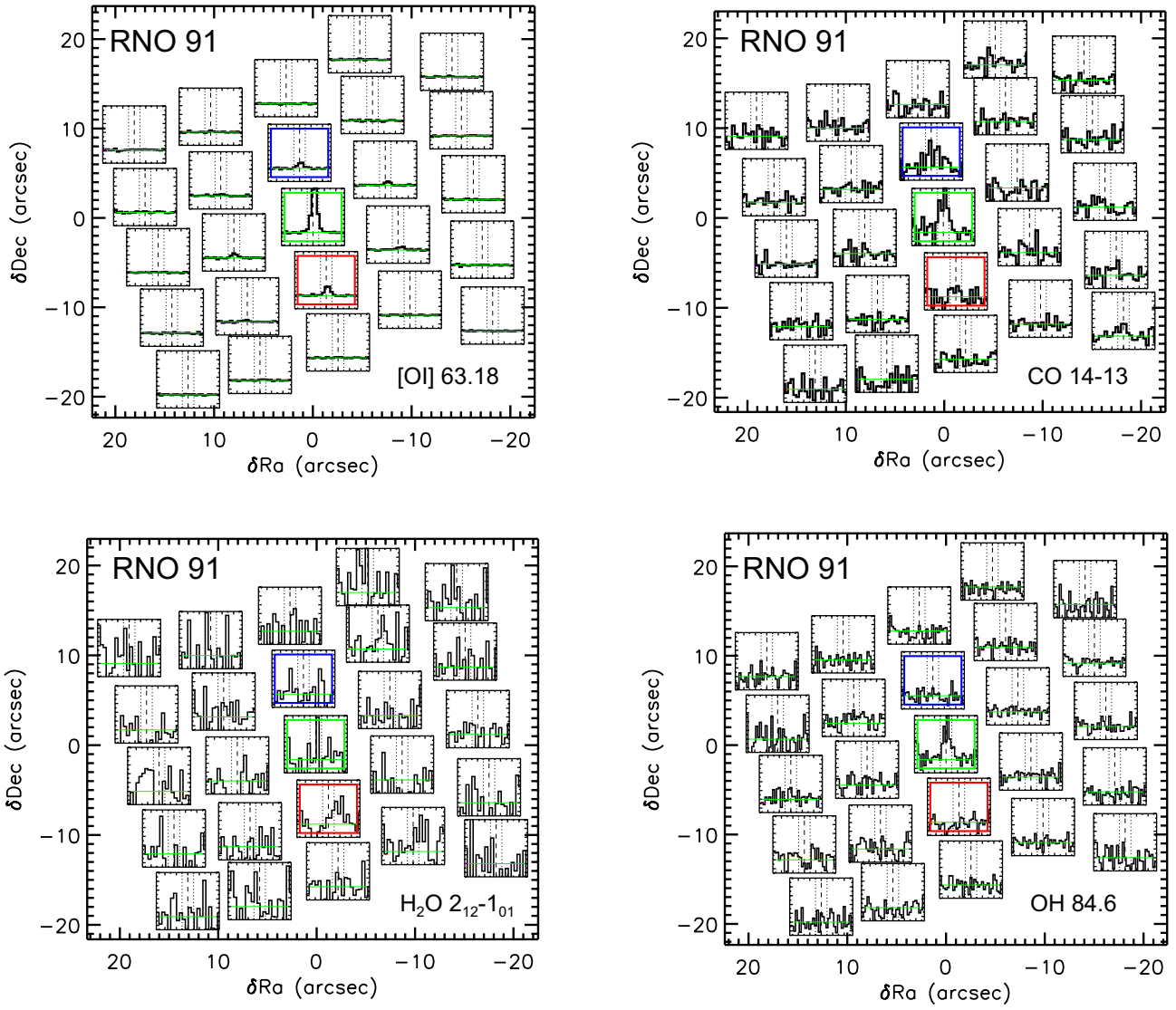
Fig. J.16. RNO91 maps in the [O I] ^3\text{P}_1 - ^3\text{P}_2 line at 63.2 \mu\text{m} , the H 2 O 2_{12} - 1_{01} line at 179.5 \mu\text{m} , the CO 14–13 at 186.0 \mu\text{m} , and the OH ^2\Pi_{3/2} J = 7/2 - 5/2 line at 84.6 \mu\text{m} .
