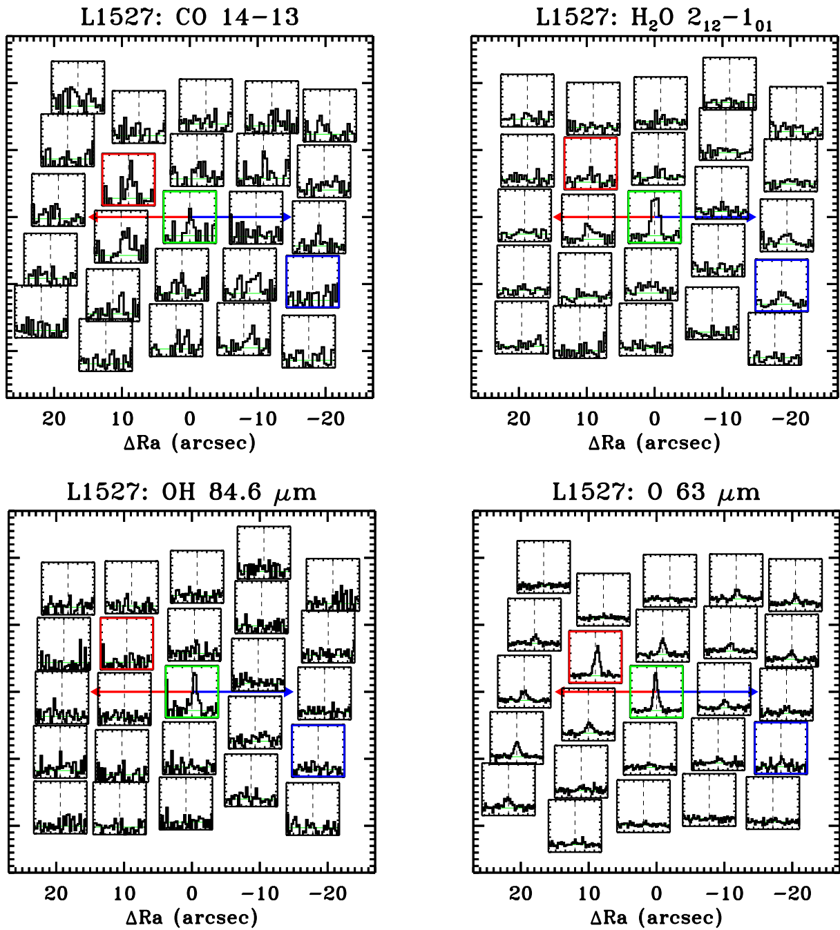
Fig. J.2. L1527 maps in the [O I] ^3\text{P}_1\text{-}^3\text{P}_2 line at 63.2 \mu\text{m} , the H 2 O 2 12 -1 01 line at 179.5 \mu\text{m} , the CO 14-13 at 186.0 \mu\text{m} , and the OH ^2\Pi_{3/2} J = 7/2\text{-}5/2 line at 84.6 \mu\text{m} .
