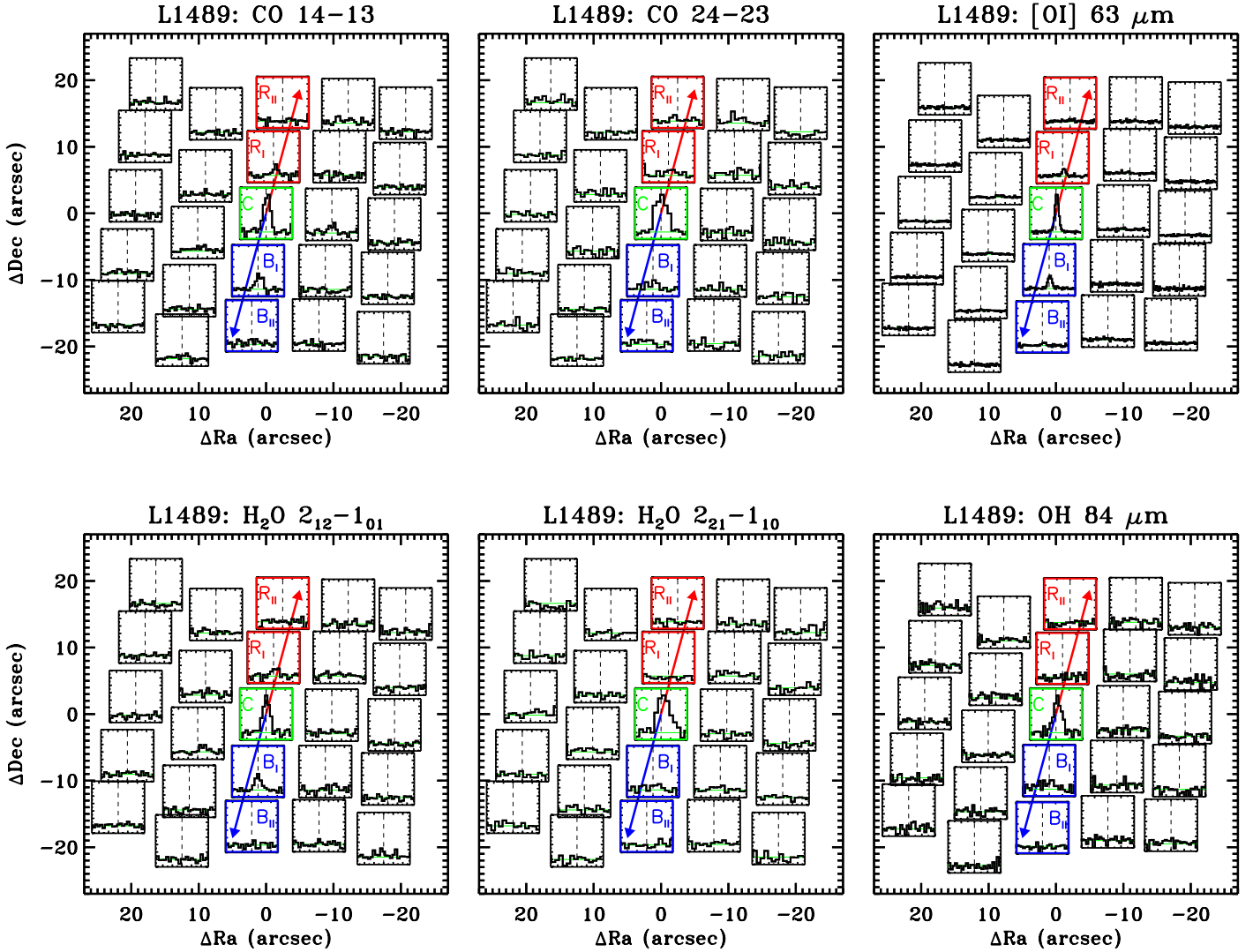
Fig. 4. The same as Fig. 3 but for the Class I source L1489.
