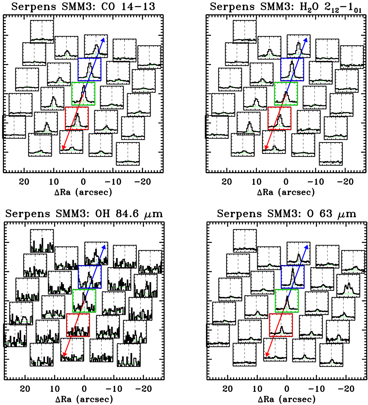
Fig. J.9. Ser SMM3 maps in the [O I] ^3\text{P}_1-^3\text{P}_2 line at 63.2 \mu\text{m} , the H 2 O 2 12 -1 01 line at 179.5 \mu\text{m} , the CO 14-13 at 186.0 \mu\text{m} , and the OH ^2\Pi_{3/2} J = 7/2-5/2 line at 84.6 \mu\text{m} .
