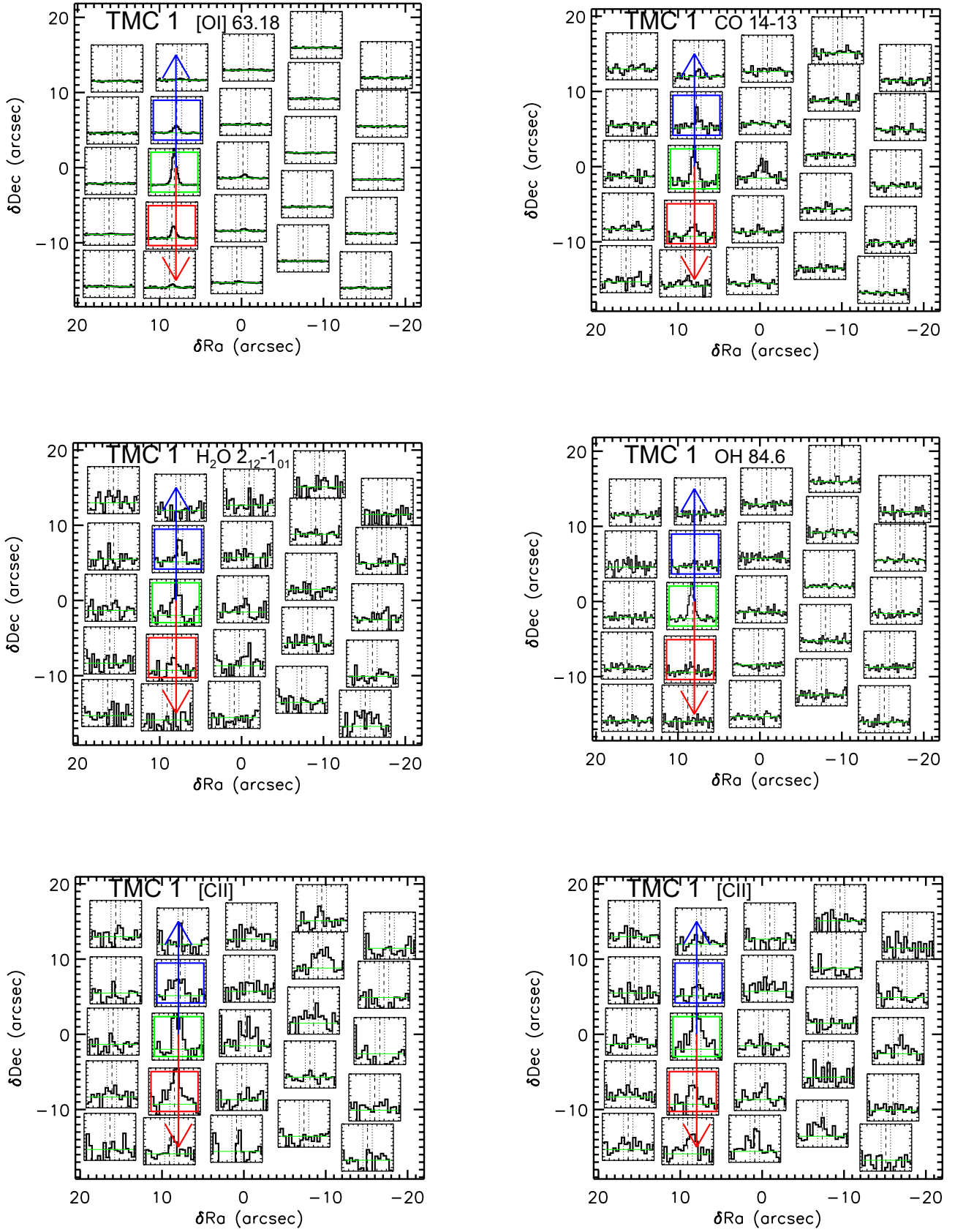
Fig. J.14. TMC1 maps in the [OI] ^3P_1-^3P_2 line at 63.2 \mu\text{m} , the \text{H}_2\text{O } 2_{12}-1_{01} line at 179.5 \mu\text{m} , the CO 14–13 at 186.0 \mu\text{m} , and the OH ^2\Pi_{3/2} J = 7/2-5/2 line at 84.6 \mu\text{m} . At the bottom, two nodes of [C II] observations are shown.
