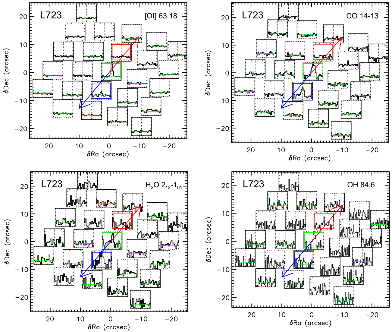
Fig. J.10. L723 maps in the [OI] ^3P_1-^3P_2 line at 63.2 \mu\text{m} , the \text{H}_2\text{O } 2_{12}-1_{01} line at 179.5 \mu\text{m} , the CO 14–13 at 186.0 \mu\text{m} , and the OH ^2\Pi_{3/2} J = 7/2-5/2 line at 84.6 \mu\text{m} .
