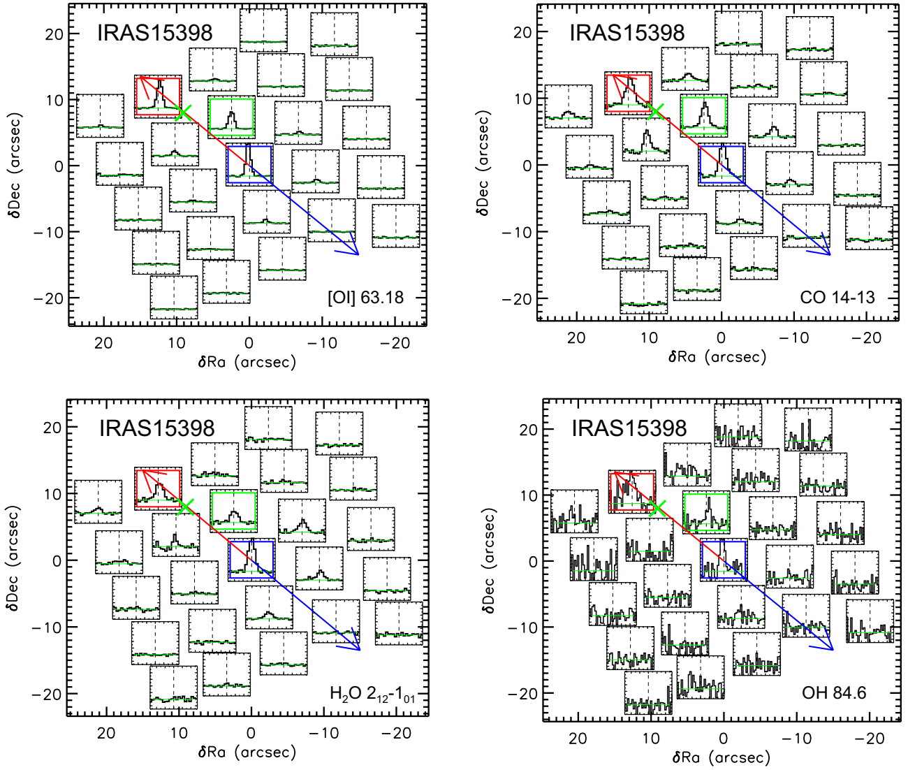
Fig. J.5. IRAS 15398 maps in the [O I] ^3P_1-^3P_2 line at 63.2 \mu m , the H 2 O 2 12 -1 01 line at 179.5 \mu m , the CO 14-13 at 186.0 \mu m , and the OH ^2\Pi_{3/2} J = 7/2-5/2 line at 84.6 \mu m . Green cross shows the on-source position.
