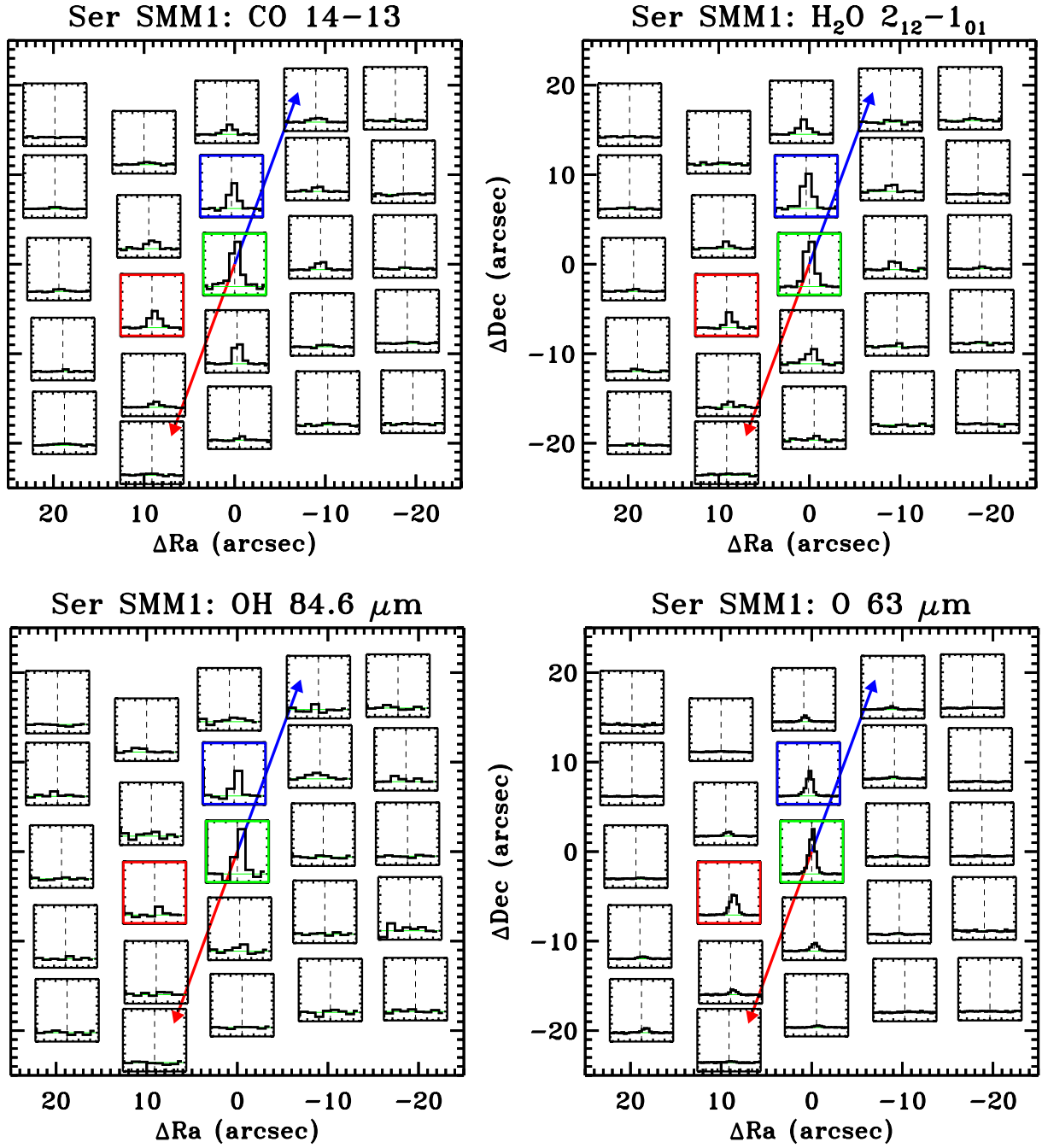
Fig. J.7. Ser SMM1 maps in the [O I] ^3\text{P}_1 - ^3\text{P}_2 line at 63.2 \mu\text{m} , the H 2 O 2 12 -1 01 line at 179.5 \mu\text{m} , the CO 14-13 at 186.0 \mu\text{m} , and the OH ^2\Pi_{3/2} J = 7/2 - 5/2 line at 84.6 \mu\text{m} .
