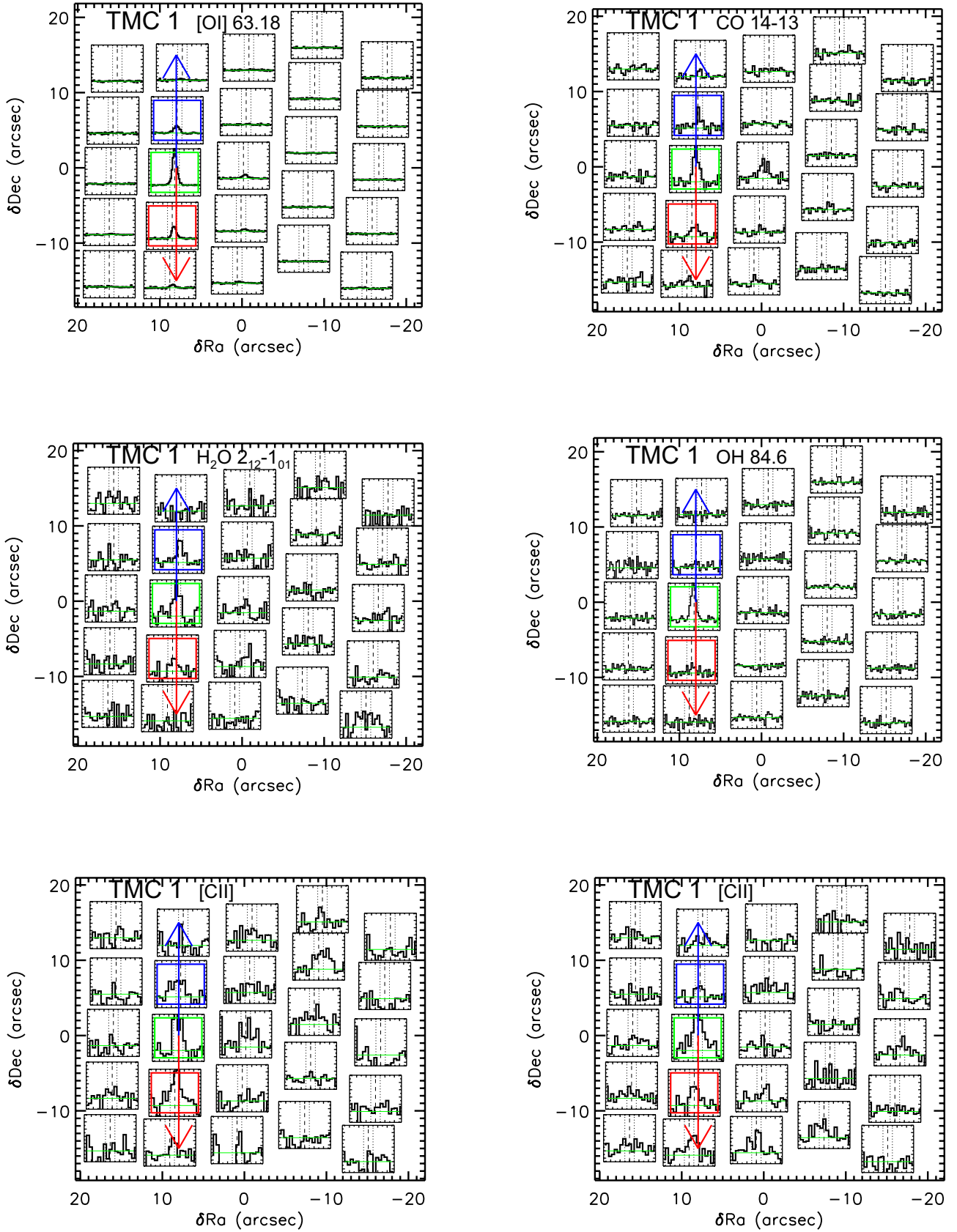
Fig. J.14. TMC1 maps in the [OI] ^3\text{P}_1-^3\text{P}_2 line at 63.2 \mu\text{m} , the \text{H}_2\text{O } 2_{12}-1_{01} line at 179.5 \mu\text{m} , the CO 14–13 at 186.0 \mu\text{m} , and the OH ^2\Pi_{3/2} J = 7/2-5/2 line at 84.6 \mu\text{m} . At the bottom, two nodes of [C II] observations are shown.
