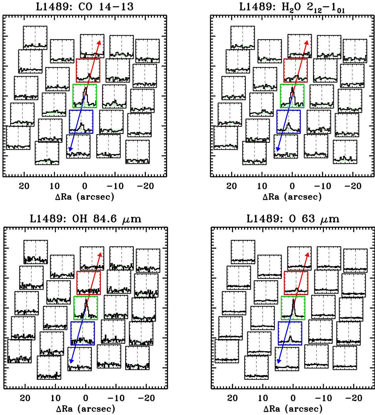
Fig. J.11. L1489 maps in the [O I] ^3P_1-^3P_2 line at 63.2 \mu\text{m} , the H 2 O 2 12 -1 01 line at 179.5 \mu\text{m} , the CO 14-13 at 186.0 \mu\text{m} , and the OH ^2\Pi_{3/2} J = 7/2-5/2 line at 84.6 \mu\text{m} .
