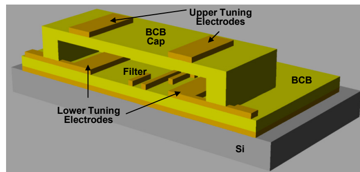
Figure 1. Cross-section of the proposed tunable bandpass filter.
