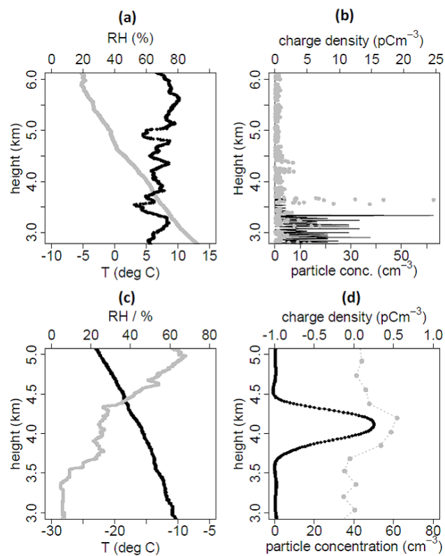
Fig. 5 Vertical profiles from balloon borne instruments through an elevated layer of Saharan dust over the Cape Verde isles ((a) and (b) taken from Nicoll et al. (2011)), and a volcanic ash plume over Scotland ((c) and (d), adapted from Harrison et al. (2010)). (b) and (d) show particle number concentration (black) and charge density (grey) measured by a disposable balloon borne aerosol counter and space charge sensor respectively. (a) and (c) show meteorological profiles of temperature (T, grey) and relative humidity (RH, black) to demonstrate that the particle and charge measurements are not related to the environmental conditions in which the sensors operate, and in particular that no liquid water cloud is present.
