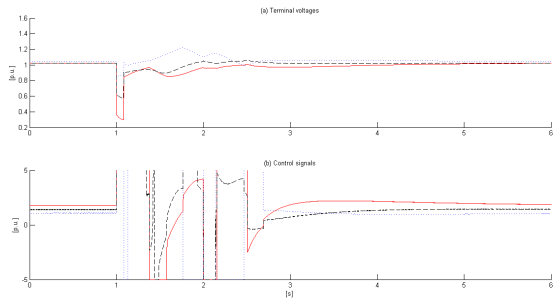
Fig. 2. Proposed controller [G1 (dot), G2 (solid), G3 (dash)]: a) V_{ti} ; b) u_{fi} .
