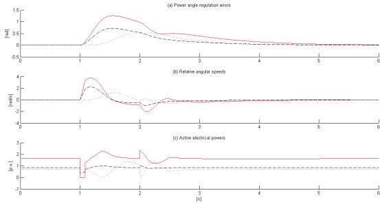
Fig. 1. Proposed controller [G1 (dot), G2 (solid), G3 (dash)]: a) \delta_i - \delta_{is} ; b) \omega_i ; c) P_{ei} .
