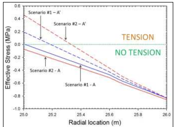
Figure 16. Radial distribution of effective stress for scenarios #1 and #2 at first and second pressure minimums during the first seasonal cycle.
