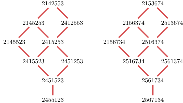
FIGURE 5. The Baxter equivalence class of the word u := 2415253 and of the permutation 2516374 = \text{std}(u) . Edges represent Baxter adjacency relations.
