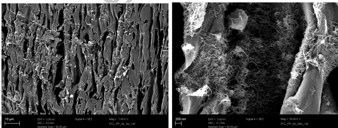
Figure 2: Morphology of PCL-3 wt.% MWNT/PP = 50/50 blends; extruded granules, PCL selectively etched using chloroform (PP phase is remaining) at two different magnifications
