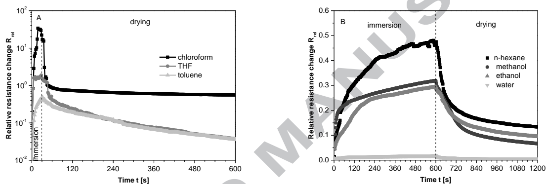
Figure 6: Relative resistance changes of PCL-3 wt.% MWNT/PP = 50/50 blends on contact with various solvents; A: good solvents, B: poor solvents
