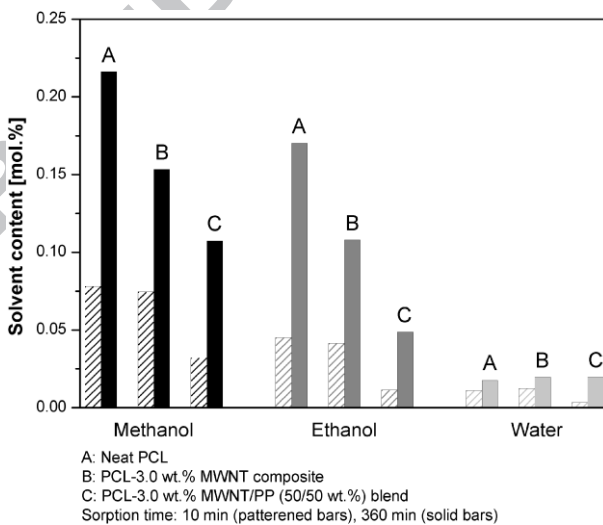
Figure 4: Solvent uptake of neat PCL (A), PCL-3.0 wt.% MWNT (B), and PCL-3 wt.% MWNT/PP = 50/50 blends (C) after immersion in ethanol, methanol, and water for 10 and 360 min
