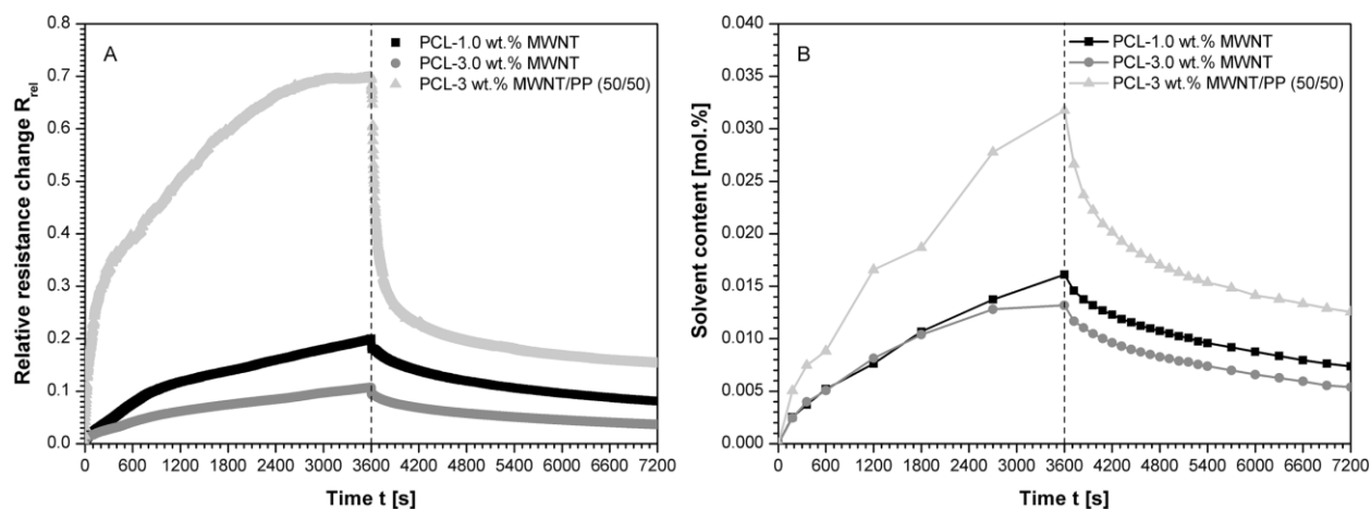
Figure 10: PCL filled with 1.0 and 3.0 wt.% MWNT and PCL-3 wt.% MWNT/PP = 50/50 blend composite in n-hexane; A: Relative resistance changes, B: sorption/desorption behaviour
