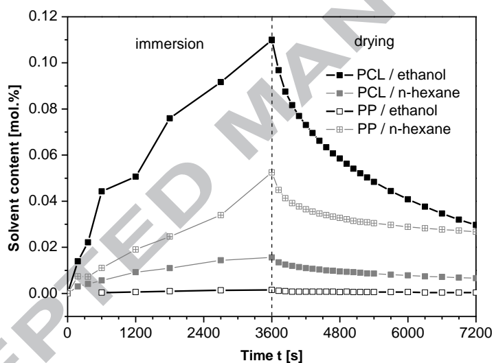
Figure 11: Solvent sorption/desorption behaviours of PCL and PP disks in ethanol and n-hexane
