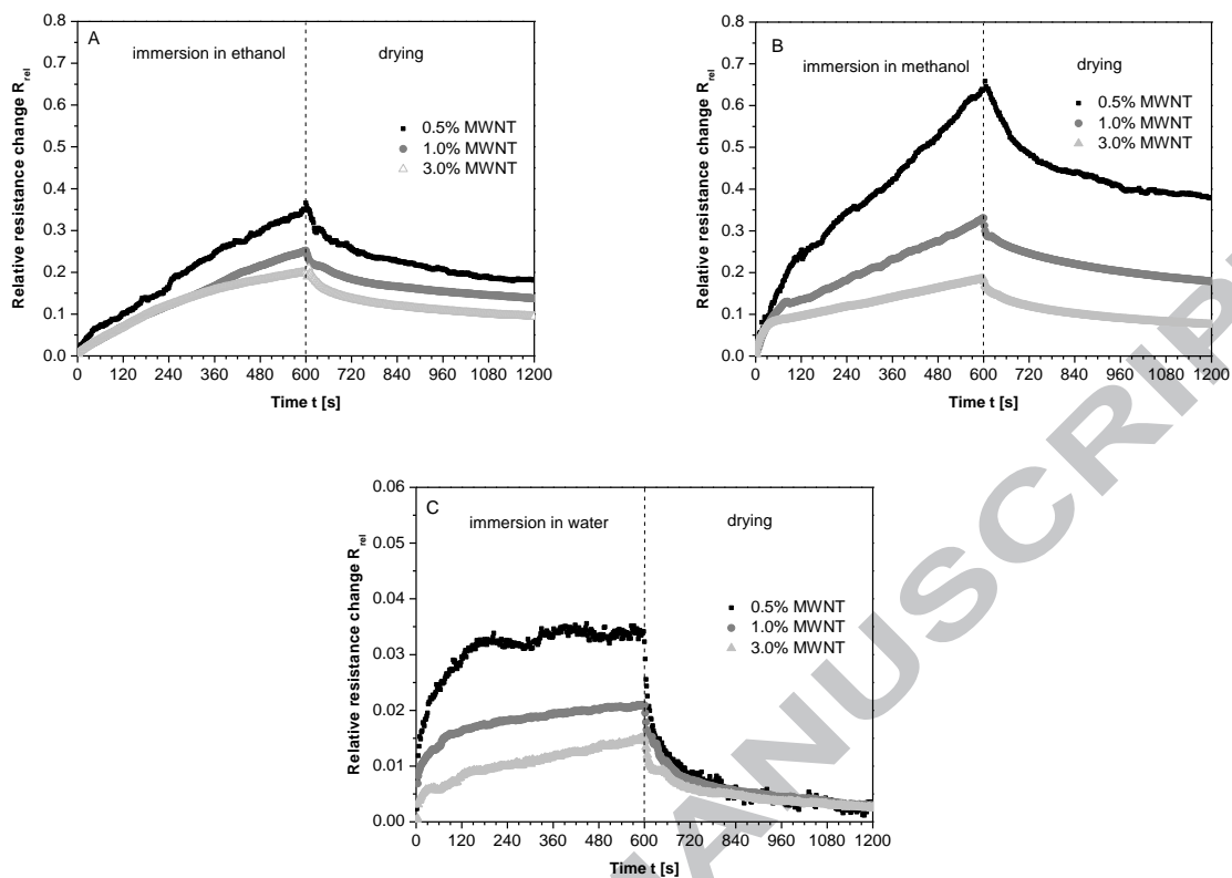
Figure 3: Relative resistance changes of PCL-MWNT disks with different MWNT loadings in poor solvents; A: ethanol, B: methanol, C: water
