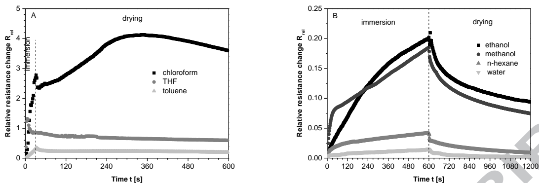
Figure 5: Relative resistance changes of PCL-3 wt.% MWNT on contact with various solvents; A: good solvents, b: poor solvents
