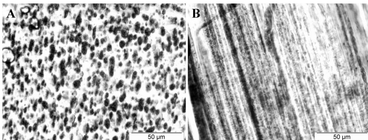
Figure 12: Morphology of a melt-drawn filament of PCL-3 wt.% MWNT/PP = 50/50 blend; A: perpendicular to the filament axis, B: parallel to the filament axis
