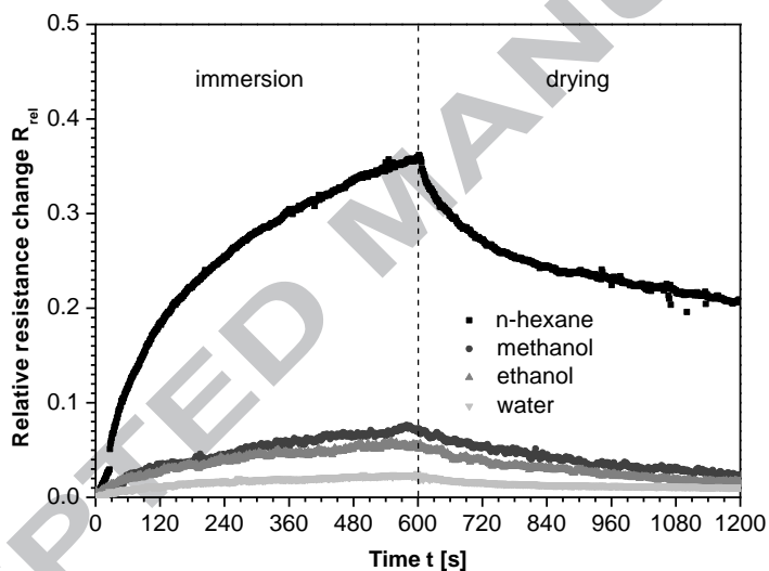
Figure 13: Relative resistance changes of melt-drawn filaments of PCL-3 wt.% MWNT/PP = 50/50 blends on contact with poor solvents
