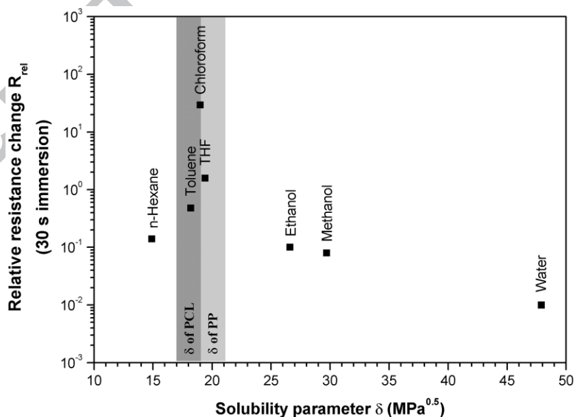
Figure 6: Relative resistance changes of PCL-3 wt.% MWNT/PP = 50/50 blends on contact with various solvents; A: good solvents, B: poor solvents
