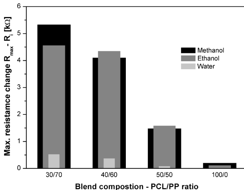
Figure 8: Maximum resistance changes of PCL-3 wt.% MWNT/PP blend composite disks with different blend composition on solvent contact of methanol, ethanol, and water; R max : maximum resistance after 10 min solvent immersion, R i : initial resistance before immersion
