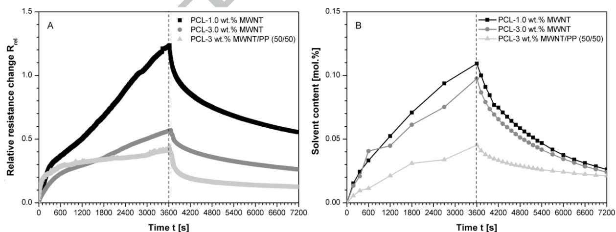
Figure 9: PCL filled with 1.0 and 3.0 wt.% MWNT and PCL-3 wt.% MWNT/PP = 50/50 blend composite in ethanol; A: Relative resistance changes, B: sorption/desorption behaviour
