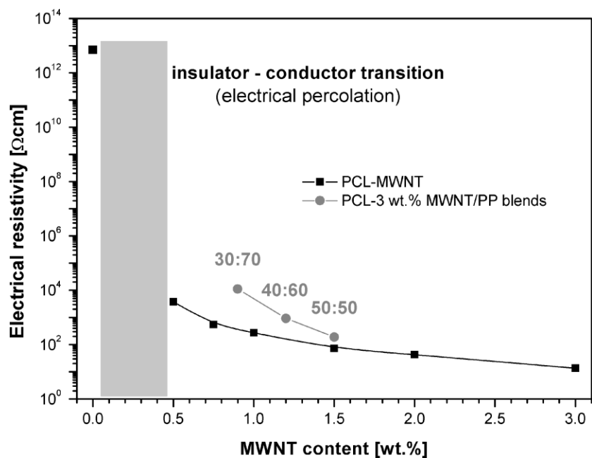
Figure 1: Electrical resistivity of PCL/MWNT composites and PCL-3 wt.% MWNT/PP blend composites
