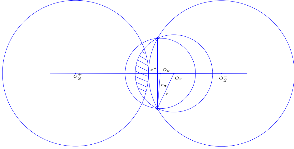
Figure 3: First construction for Lemma 4
