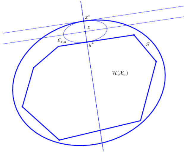
Figure 1: Construction of an empty ellipsoid for Lemma 1
