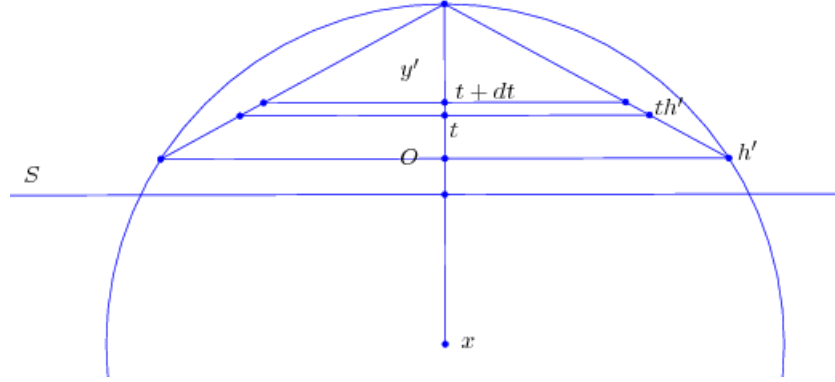
Figure 7: Probability integration in a lens
