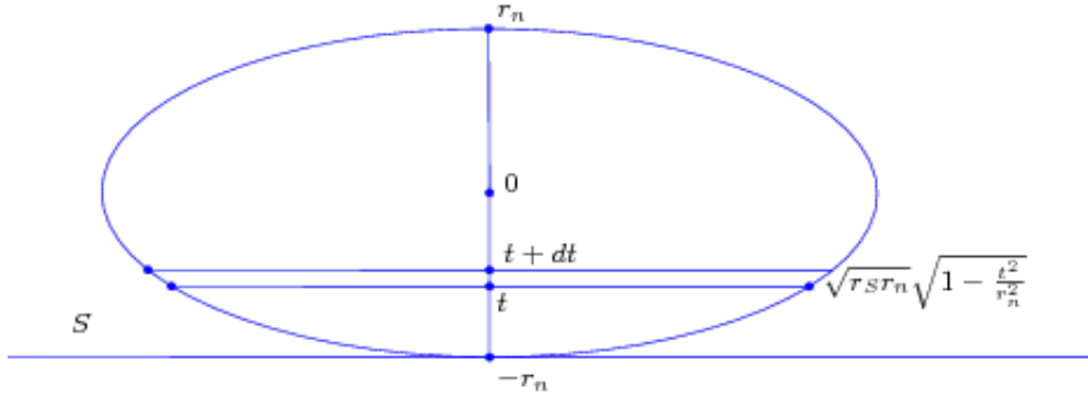
Figure 5: Probability integration in an ellipsoid
