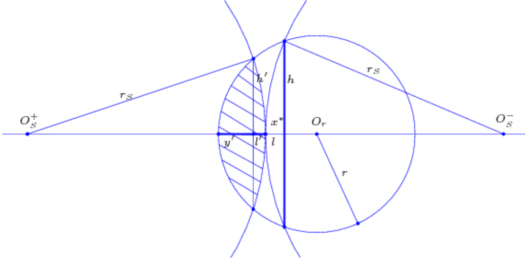
Figure 4: Definition of some useful lengths for Lemma 4
