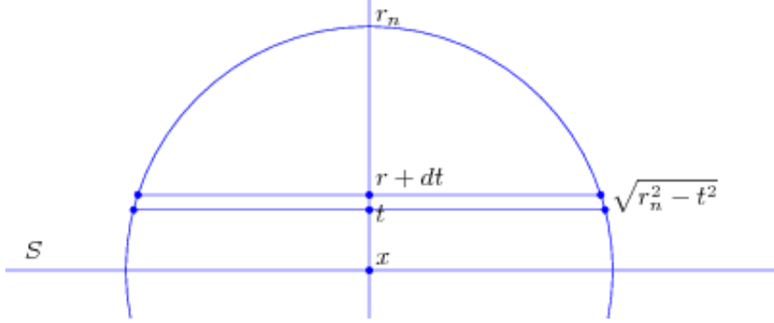
Figure 6: Probability integration in a disc
