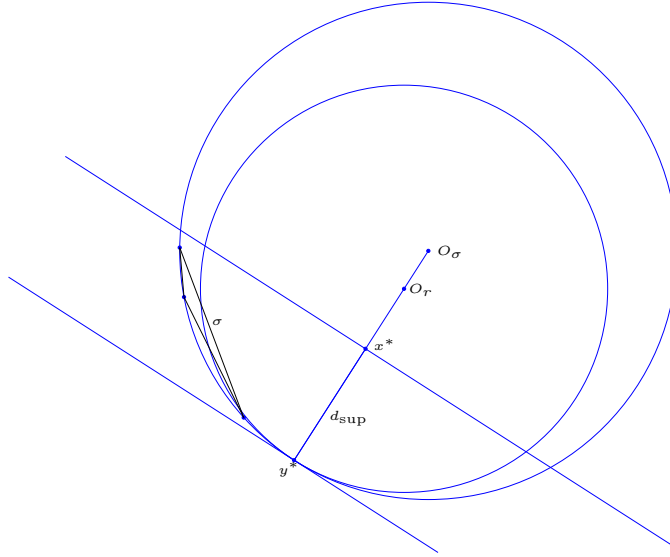
Figure 2: Construction of an empty \mathcal{C} for Lemma 2
