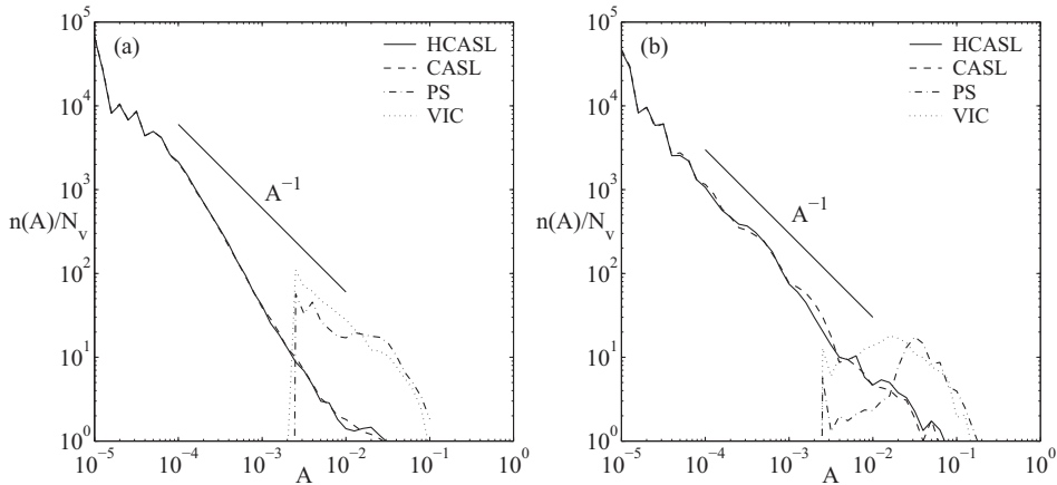
Fig. 9. Time-averaged vortex number density n(A) normalised by the total number of vortices N_v versus area A for the four algorithms. Curves correspond to data collected on the period (a) t \in [10, 100] and (b) t \in [100, 500] .
