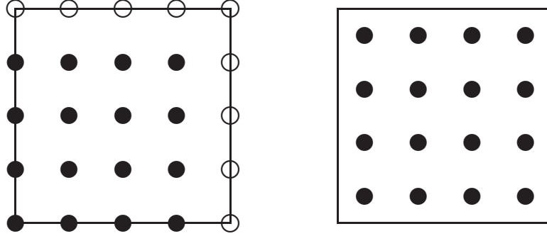
Fig. 3. Two distinct point vortex placements within a grid box for m = 4 . The black square denotes the grid box and the filled circles correspond to point vortices within the grid box while the unfilled ones represent periodic point vortices belonging to the neighbouring grid boxes.
