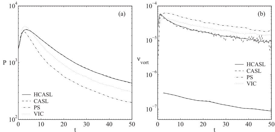
Fig. 7. Early evolution of (a) the palinstrophy P and (b) the vorticity diffusion coefficient \nu_{\text{vort}} . In figure (b) \nu_{\text{vort}} has been computed on the inversion grid (upper curves) for the four algorithms, and on the recontouring grid (lower curves) for HCASL and CASL.
