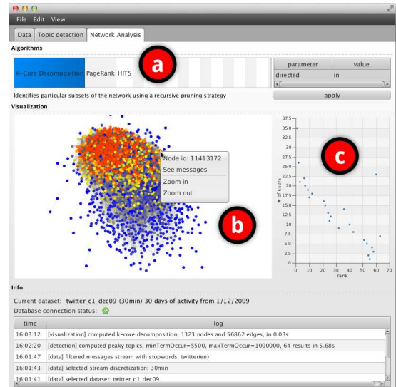
Figure 4: Visualizing a network of authors about a selected topic, colored with k -shells.
