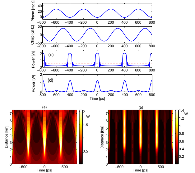
Figure 7: As in Fig. 6, with input sinusoidal phase modulation. (a) total power; (b) power after bandpass filtering; (c) unfiltered or (d) filtered output pulse train profile at 3 km of DCF;
