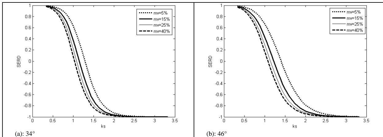
Fig. 11. Behaviour of the SERD from the IEM data as a function of the soil moisture and ks. F=5.3GHz, Exponential autocorrelation function, incidence angles =34° and 46°.
