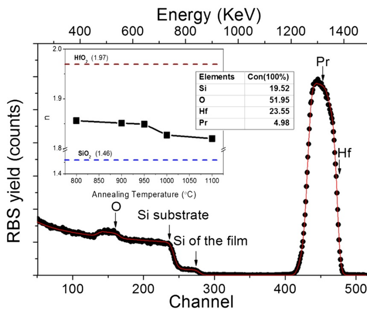
Figure 1 Experimental RBS spectrum (points) and simulated curve using SIMNRA (solid line) for as-deposited film. Inset table is the chemical composition of the film. Inset figure is the refractive index evolution versus T_A . The pure HfO 2 and pure SiO 2 indices are also shown in dashed lines. The films are about 170 nm in thickness.
