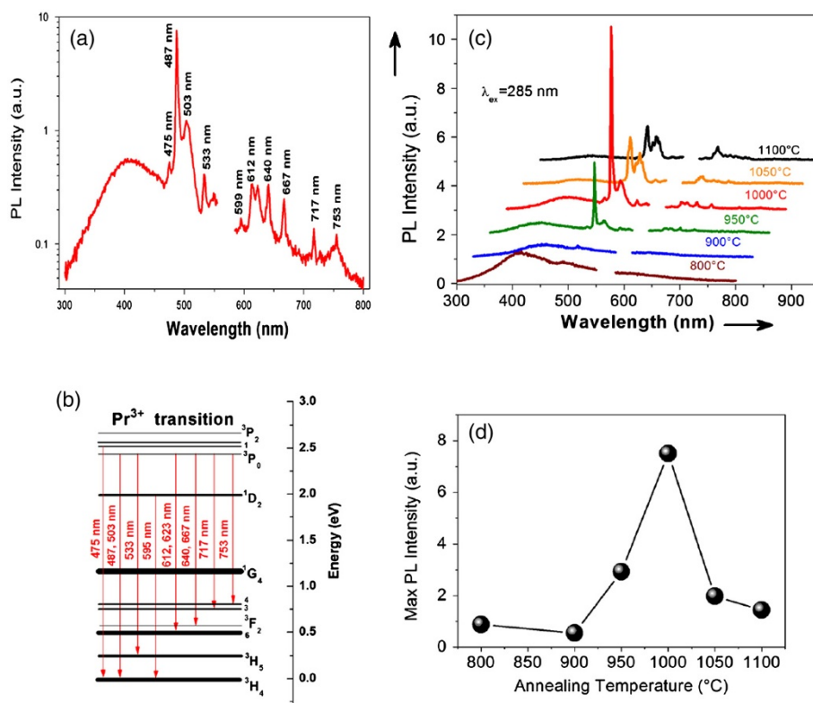
Figure 4 PL spectra, schematics, and PL behavior. (a) PL spectrum in logarithmic scale for 1,000°C annealed layer. (b) The schematics of the \text{Pr}^{3+} intra-4f transitions. (c) PL spectra of the films annealed at different annealing temperatures ( T_A = 800^\circ\text{C} to 1,100^\circ\text{C} ). The excitation wavelength is 285 nm. (d) The behavior of the PL intensity of the ^3\text{P}_0 \rightarrow ^3\text{H}_4 transition at 487 nm with T_A .
