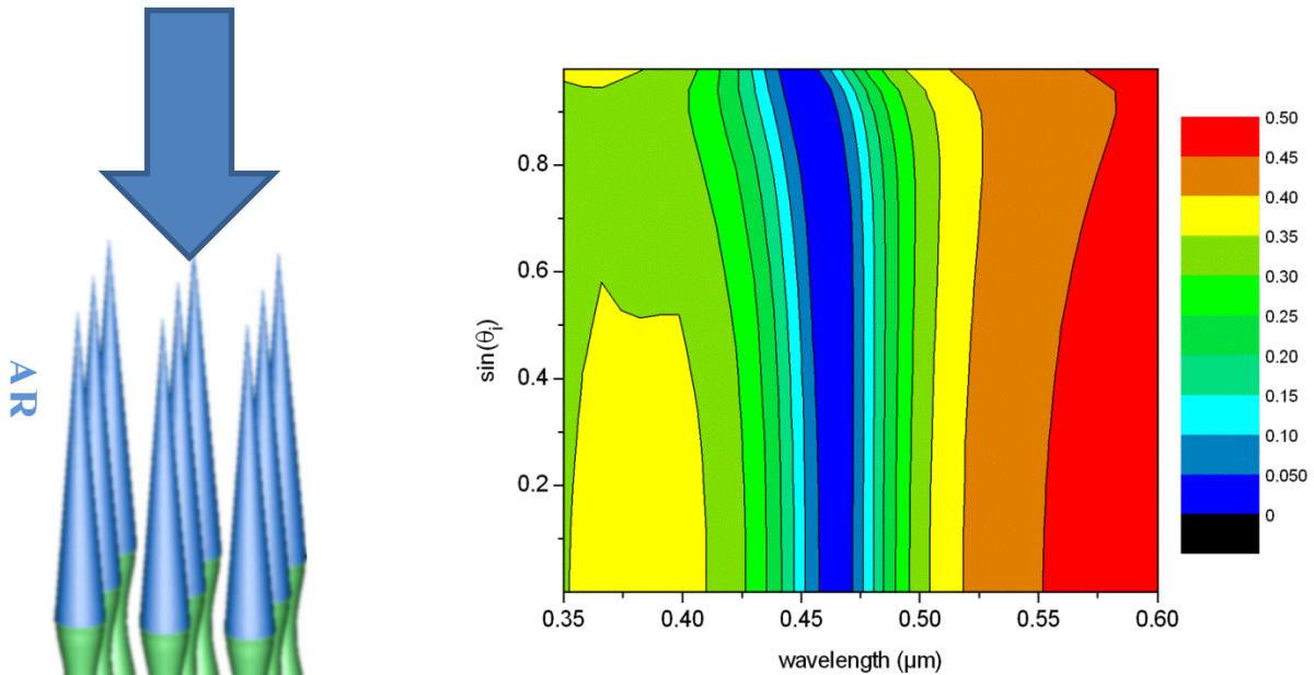
Fig.1.21. Reflectivity of the crossed grating in Fig.1.19 as a function of the wavelength and of the sine of the incident angle. Period d = 3 nm, system thickness h = 6.2 nm, filling factor = 0.7, i.e. c/d = 0.837 .
