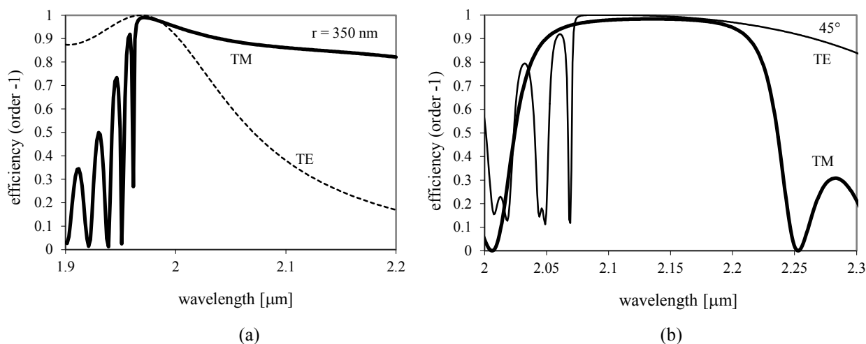
Fig.1.25. Diffraction efficiency in order -1 as a function of the wavelength lying inside the band gap. (a) r = 350 \text{ nm} , (b) r = 150 \text{ nm} (after [1.46] with the publisher's permission).
