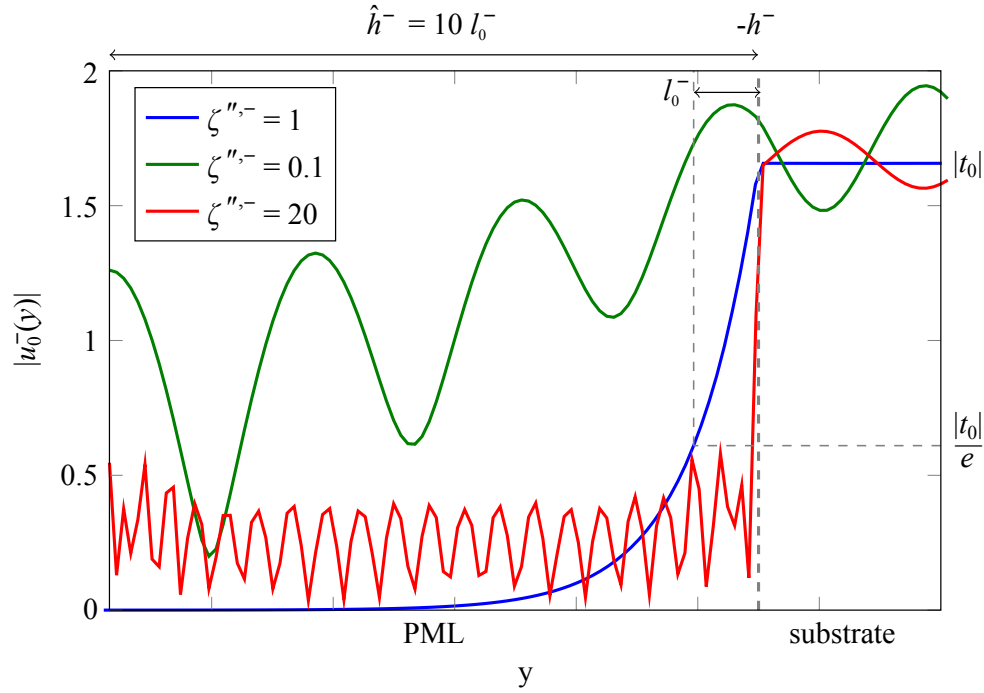
Fig. 5.9: Zero th transmitted order by a grating with a rectangular cross section (see parameters in text, part 5.2.4.2) for different values of \zeta''^- : blue line, \zeta''^- = 1 , correct damping; green line, \zeta''^- = 0.1 , underdamping; red line, \zeta''^- = 20 , overdamping.
