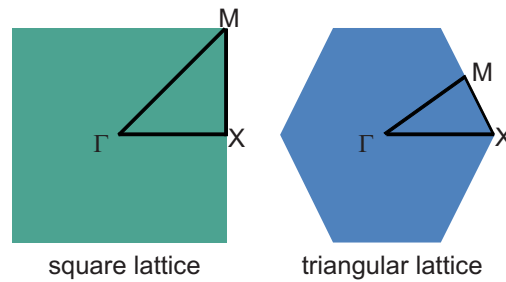
Figure 9.8: Brillouin zone
