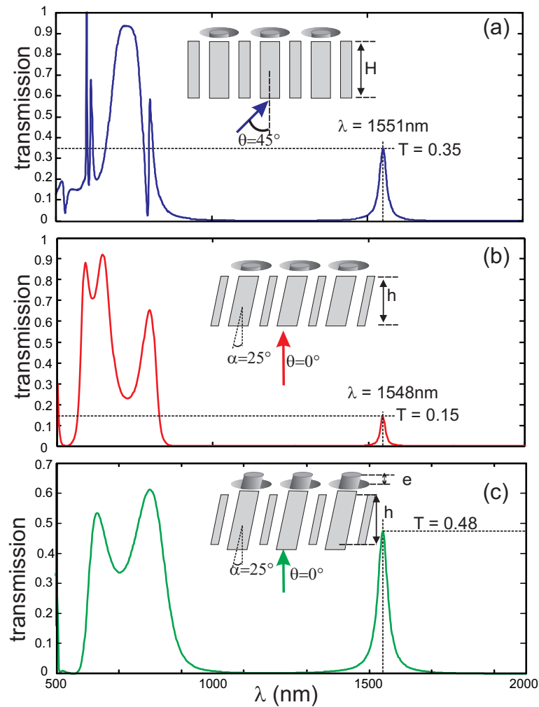
Figure 9.20: Zero-order transmission spectra for three different AAA configurations where outer and inner radii are fixed to r_e = 130 nm and r_i = 65 nm respectively. (a) Conventional structure illuminated at 45^\circ (metal thickness of h = 495 nm). (b) SAAA with tilt angle of 25^\circ with respect to the vertical direction. The thickness of the metallic film ( h = 430 nm) is chosen in order to get a TEM peak transmission at \lambda = 1550 nm. (c) SAAA structure with inner metallic parts that stretch out from the metallic film over a distance e = 80 nm. This allows increasing of the impedance matching between the in- and out-coming plane waves with the TEM guided mode inside the apertures. The metal thickness is also adjusted in order to get a TEM peak at \lambda = 1550 nm with a transmission efficiency of 48%.
