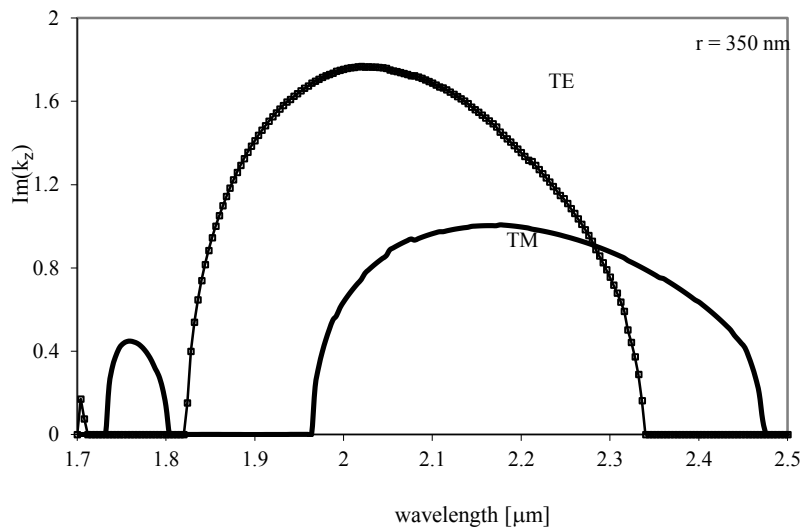
Fig.1.24. Forbidden bands for the photonic crystal made of circular cylinders with d = 1.414 μm, r = 0.35 μm (after [1.46] with the publisher's permission).
