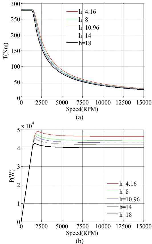
Fig. 10 (a) Torque-speed, (b) power-speed characteristics for the 3-phase PRIUS type machine for I_p = 212 A
