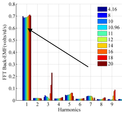
Fig. 4 No load EMF frequency spectrums for h = [4.16\text{mm}; 20\text{mm}] .
