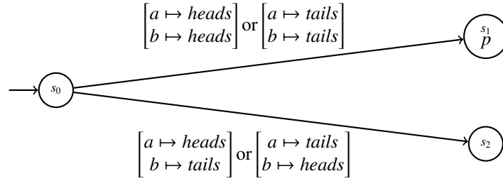
Figure 2: Model \mathcal{G}_{\llbracket \langle \rangle \rrbracket}
