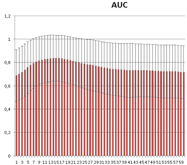
Fig. 2: AUC scores between actor’s and viewer’s saliency maps for different time-shifts (in frames)
