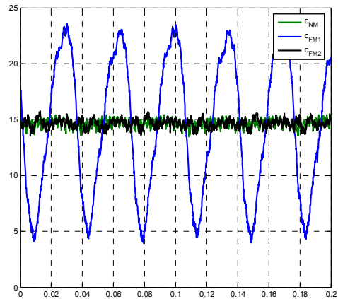
Fig. 8. Torques in normal and fault mode (Experimental Results)
