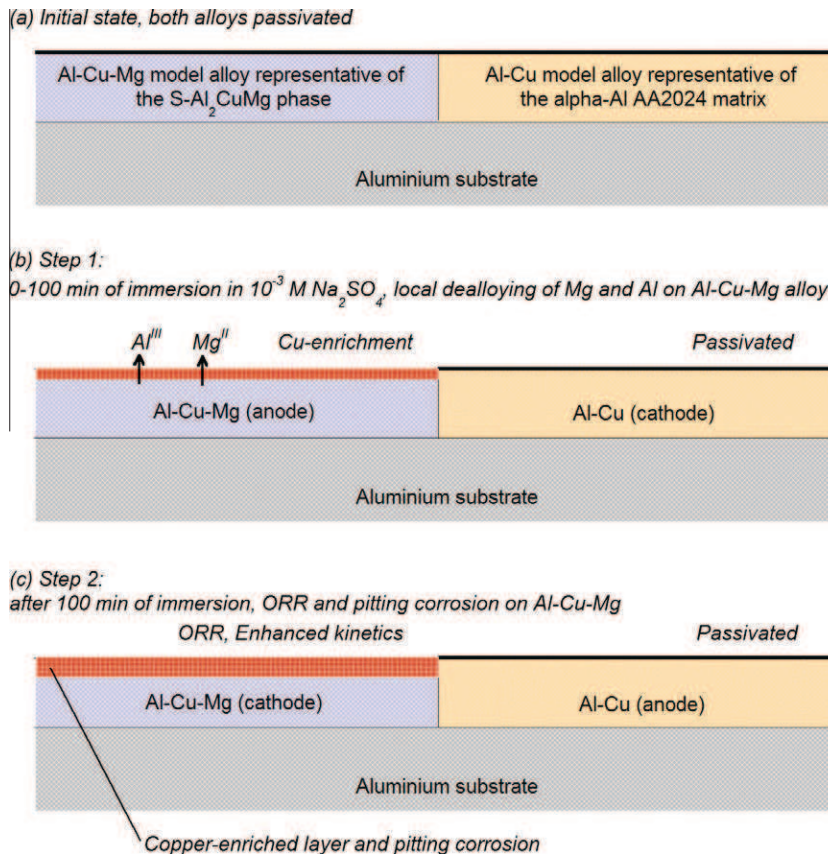
Fig. 10. Schematic diagram of the corrosion behaviour of the model couple alloy, (a) initial state, (b) Step 1, up to 100 min of immersion in 10 -3 M Na 2 SO 4 and (c) Step 2, after 100 min of immersion.
