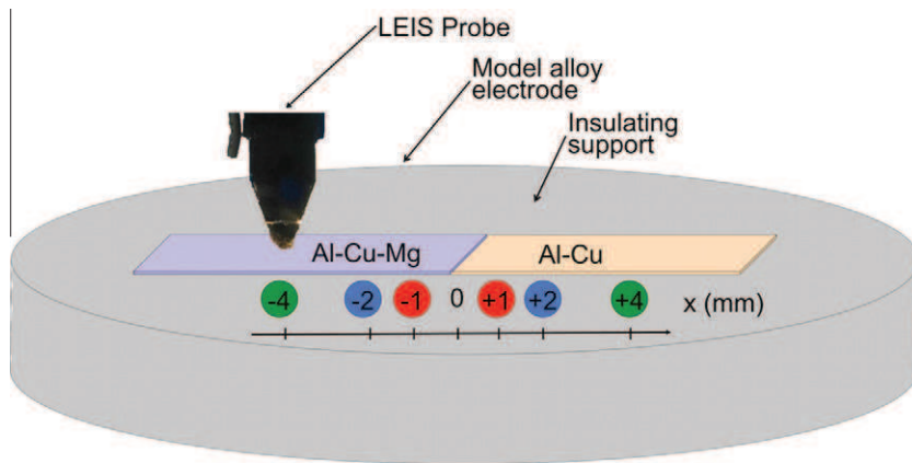
Fig. 6. Schematic representation of the different LEIS measurement locations on a model alloy electrode. The distance values are given in millimetres.
