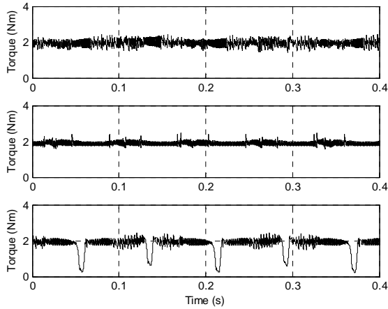
Fig. 9. Simulated torques with, from top to bottom: one phase, two non-adjacent phases and two adjacent phases open-circuited
