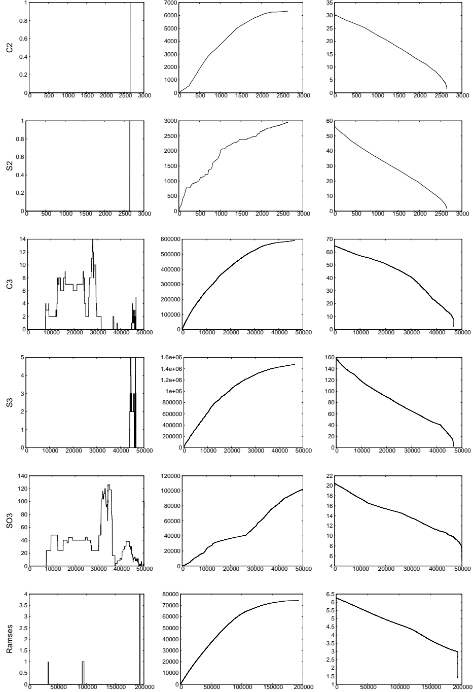
Fig. 10. We plotted as functions of i the number of blockers in the simplicial complex K_i on the left, the cumulated number of poppable blockers removed from the data structure up to step i in the middle and the average number of neighbors per vertex on the right. From top to bottom: the initial Rips complex has vertex set C_2 , S_2 , C_3 , S_3 , S_{03} , and Ramses .
