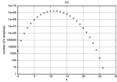
Fig. 7. Number of k -simplices in \mathcal{R}(P, r) as a function of k for a point set P that samples C_2 . We used a logarithmic scale for the y -axis. Experimentally, we observe that the number of k -simplices is above but close to \frac{n}{k+1} \binom{N}{k} for N = 25 . The number of simplices is thus at least \frac{n}{N+1} 2^N \approx 3.4 \cdot 10^9 . This should be compared with our data structure which has only to store 2646 vertices and 80304 edges to represent the same complex.
