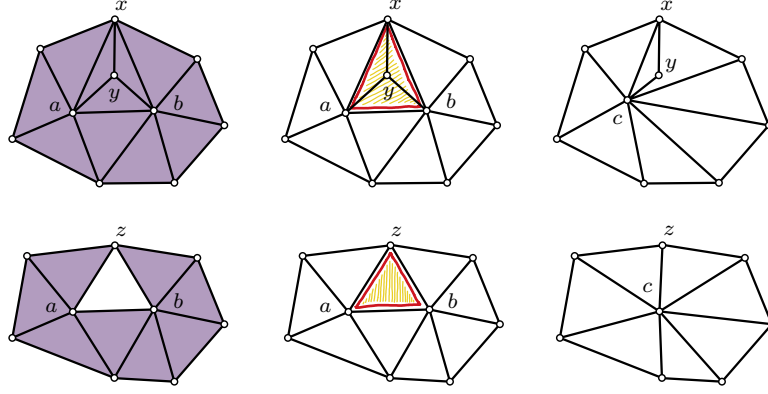
Fig. 2. Left and middle: two 2-dimensional simplicial complexes with a blocker through ab . Right: The edge contraction ab \mapsto c may (top) or may not (bottom) preserves the homotopy type.
