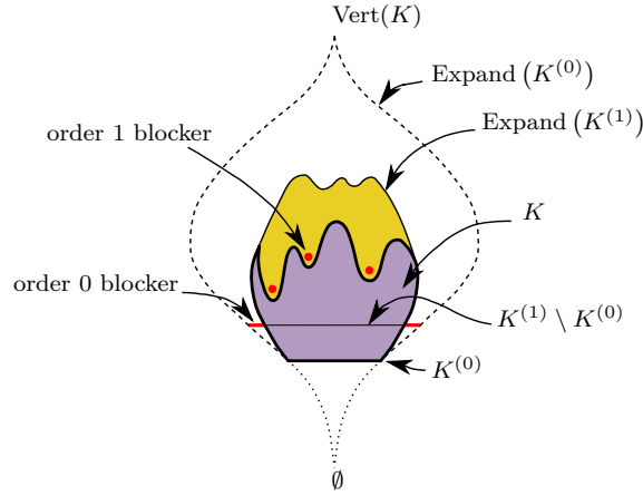
Fig. 3. Hasse diagram of K .
