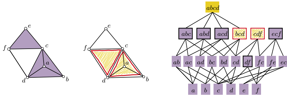
Fig. 4. Left: simplicial complex consisting of six vertices, ten edges and four non-overlapping shaded triangles. Middle: same simplicial complex represented by its 1-skeleton and order-1 blocker set \{cdf, bcd\} . Right: Hasse diagram of the expansion of the 1-skeleton. Nodes in dark gray are in the simplicial complex. Blockers and inclusion-maximal simplices are shown as framed nodes.
