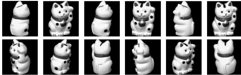
Fig. 8. Twelve of the 72 points in the dataset Lucky_cat . Each point represents a 128 pixel by 128 pixel image of a toy cat taken during its rotation around a fixed axis.
