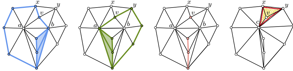
Fig. 1. From left to right: link of a , link of b , link of ab and simplicial complex after contraction of the edge ab . One can check that ab satisfies the link condition. Equivalently, no blocker contains ab (see Section 4.3). As a consequence, the contraction of ab preserves the homotopy type. Note that the edge contraction ab \mapsto c creates the blocker cxy and \alpha = x and \beta = y satisfy (i) and (ii) in Lemma 4. The contraction of any of the edges cv , xv and yv removes blocker cxy .
