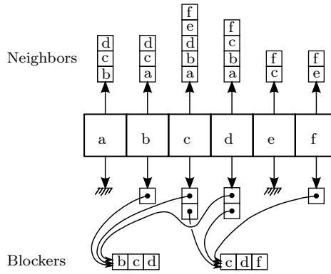
Fig. 5. Data structure representing the simplicial complex in Figure 4.
