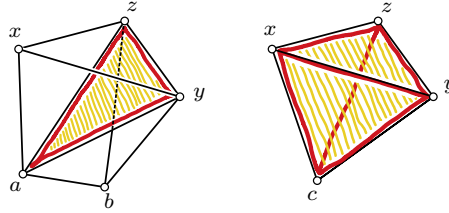
Fig. 6. Triangle ayz is a 2-blocker. We have that \text{Lk}(a) = \{x, y, z, xy, xz, b, by, bz\} , \text{Lk}(b) = \{y, z, yz, a, ay, az\} , \text{Lk}(ab) = \{y, z\} . Note that \sigma = \alpha\beta with \alpha = x and \beta = yz fulfills (i) and (ii) in Lemma 4. Therefore, the edge contraction ab \mapsto c leads to the creation of the 3-blocker xyz and the destruction of the 2-blocker ayz .
