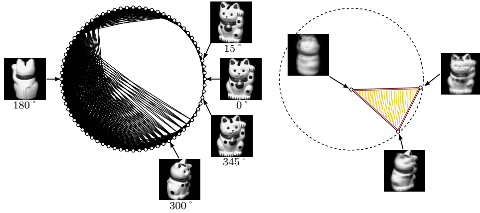
Fig. 9. Left: Rips complex of the point set Lucky_cat . Right: After simplification, we obtain a simplicial complex which consists of three vertices, three edges and has a unique blocker.
