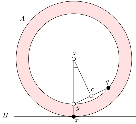
Figure 5: Notation for the proof of Lemma 9.
