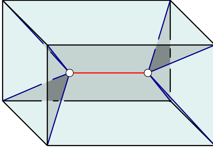
Figure 2: The box is P , and we take \varepsilon = 0 . The set \mathcal{C}^4 \subset \mathcal{AM}^4 , consisting of the centers of annuli tangent to four faces is the segment connecting the hollow dots. It has dimension one, rather than dimension zero as we would expect in the absence of degeneracy.
