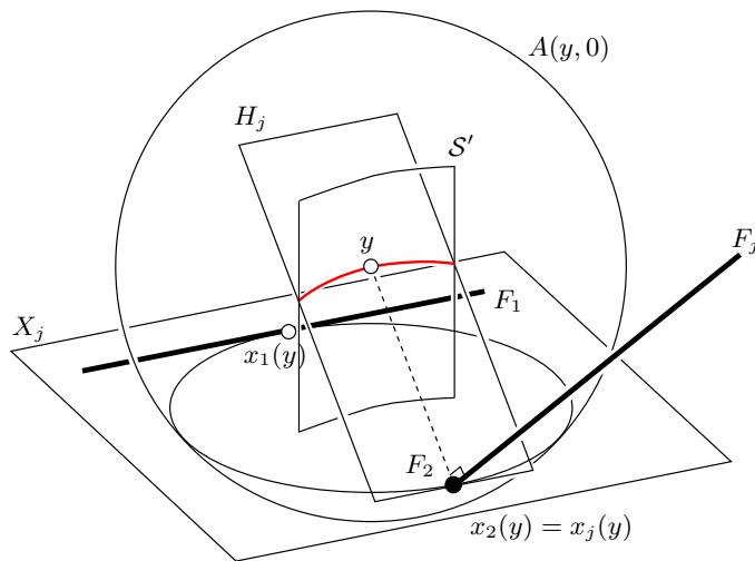
Figure 3: Notation for the proof of Lemma 5. A(y, 0) is tangent to F_1 , F_2 and F_j .
