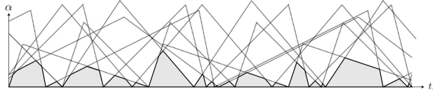
Fig. 3. Possible values for (t_i, \alpha) constrained by all tasks j \in \mathcal{G}(i)
