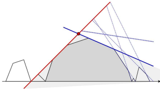
Fig. 6. The lowest intersection point of a fixed increasing line with decreasing lines
