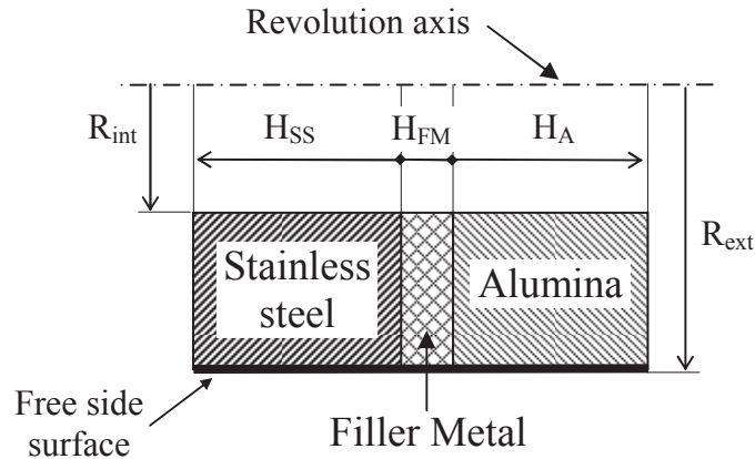
Figure 3. Geometrical parameters of the ceramic metal assembly
