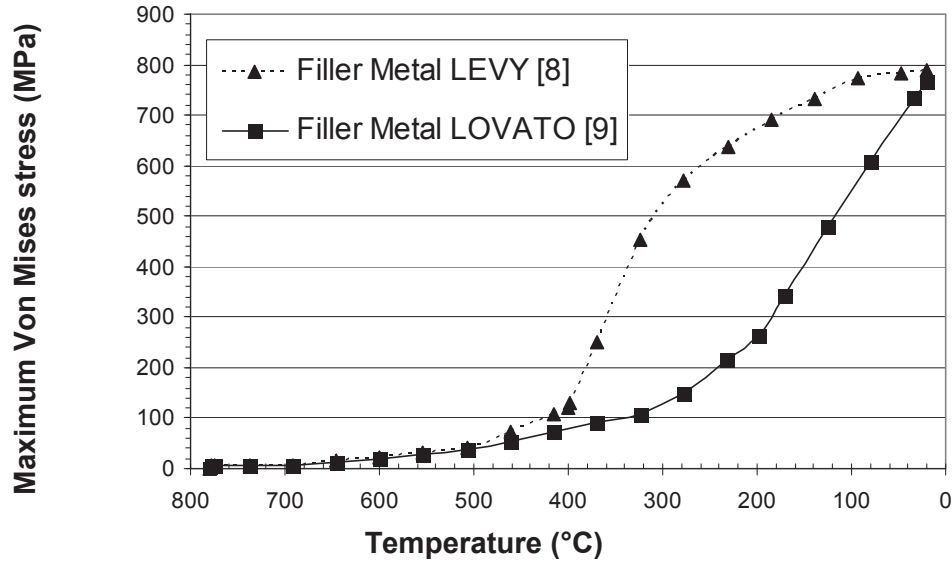
Figure 7. Maximum Von Mises stress on the free side surface according to furnace temperature and filler metal mechanical properties
